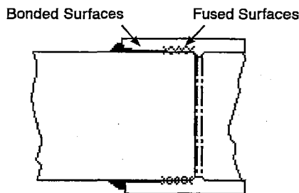
FIGURE 4 BONDED AND FUSED SURFACES OF JOINED HOSES
