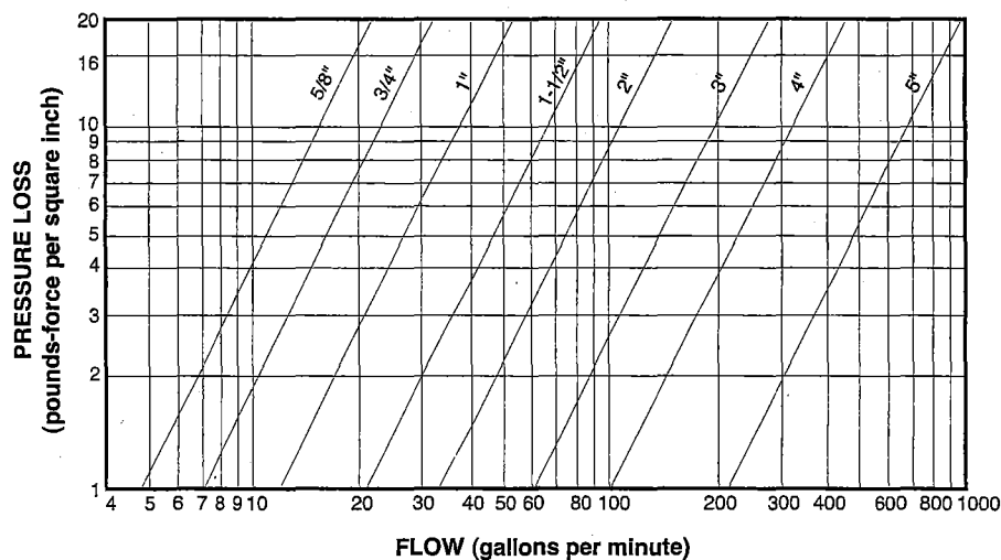
CHART A 1.2 FRICTION LOSSES FOR DISK-TYPE WATER METERS
