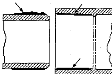
FIGURE 2 CEMENT COATINGS OF SUFFICIENT THICKNESS
