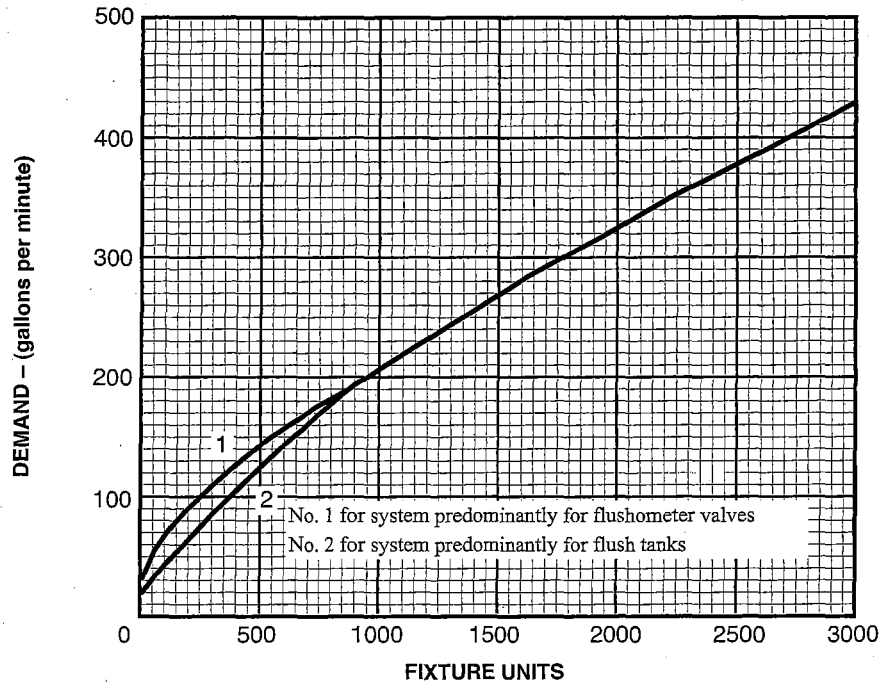
CHART A 2.1 ESTIMATE CURVES FOR DEMAND LOAD
