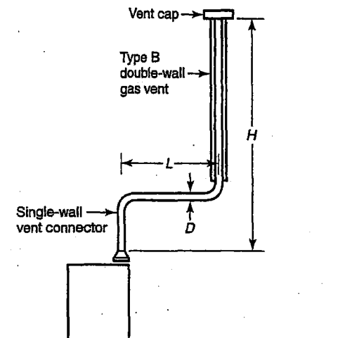
FIGURE G 1.0(a) TYPE B DOUBLE-WALL VENT SYSTEM SERVING A SINGLE APPLIANCE WITH A TYPE B DOUBLE-WALL VENT
