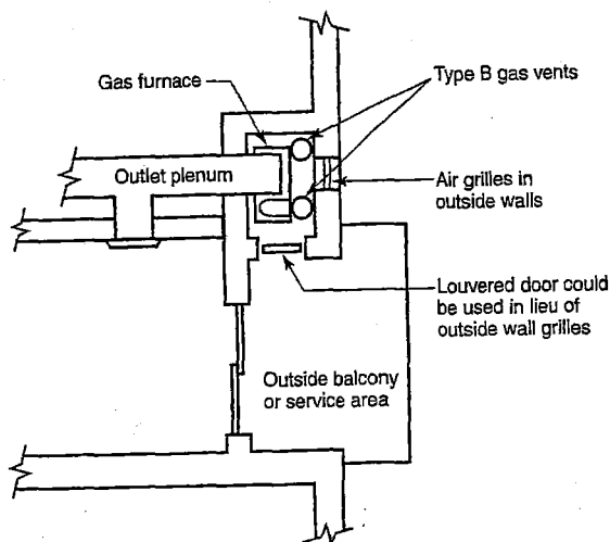
FIGURE 509.6.4.1 PLAN VIEW OF PRACTICAL SEPARATION METHOD FOR MULTISTORY GAS VENTING [NFPA 54: FIGURE 12.7.4.2]
