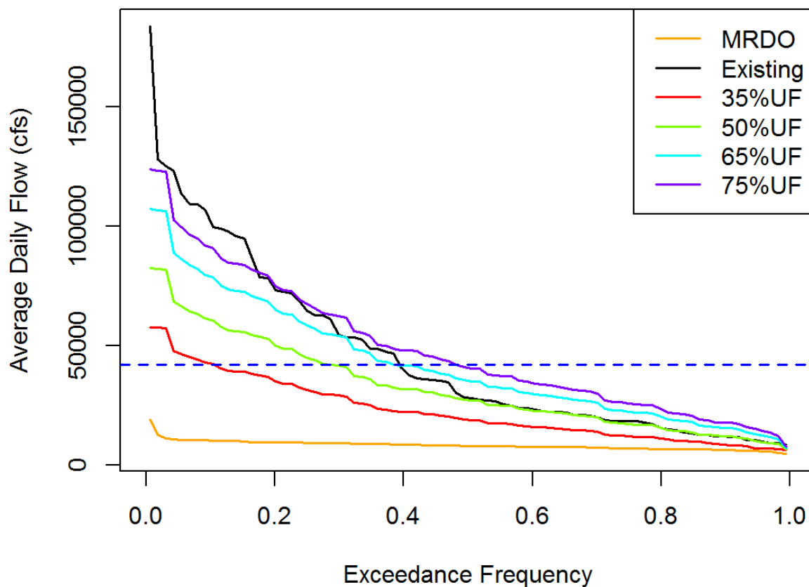
Figure 5.3-5. Frequency of Meeting January-March Delta Outflows to Benefit Adult Longfin Smelt for Minimum Required Delta Outflow (MRDO), Existing Conditions as Modeled by CalSim II, and Delta Outflows Resulting from 35% to 75% of Unimpaired Delta Inflow.
