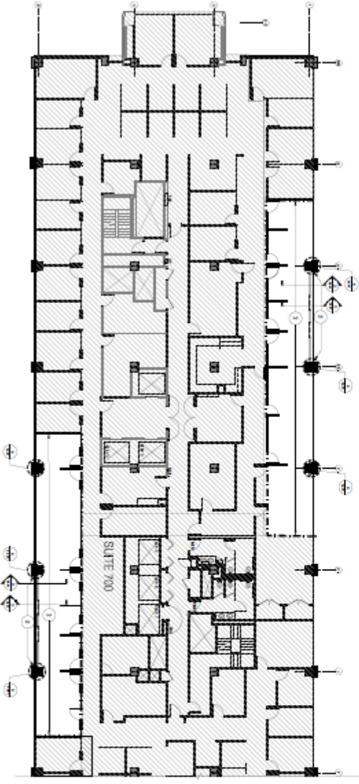
SEVENTH FLOOR CONST. PLAN
