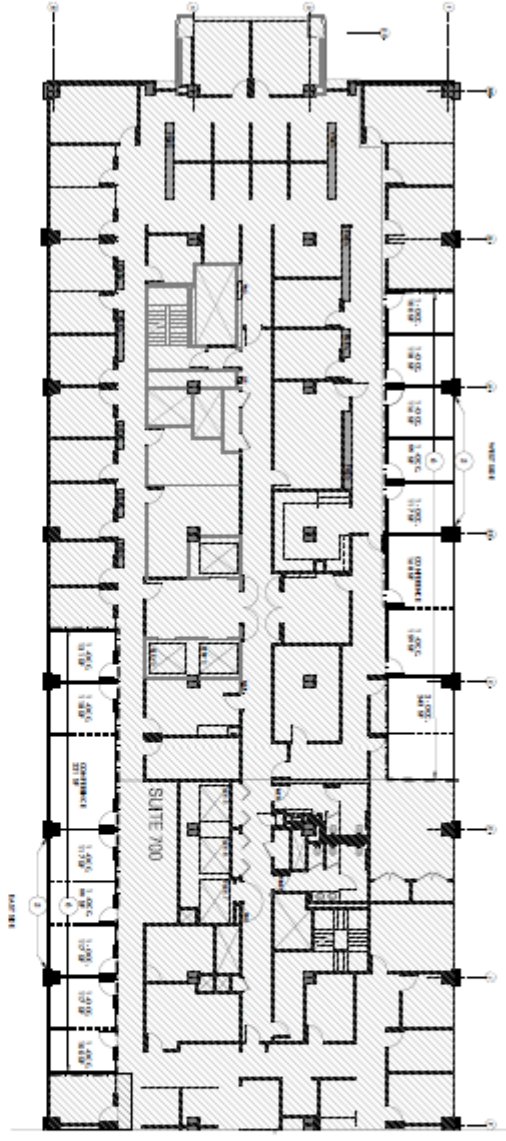
SEVENTH FLOOR DEMO PLAN
