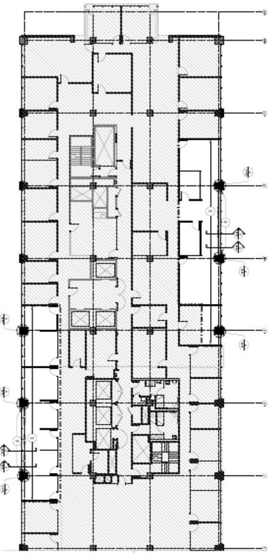
2-2. 5TH FLOOR CONST. PLAN
