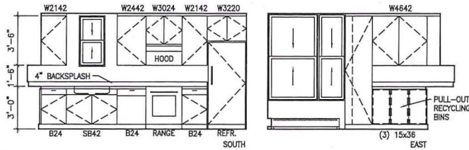
F10 House – interior elevations
