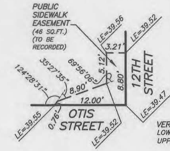
DETAIL B NO SCALE
