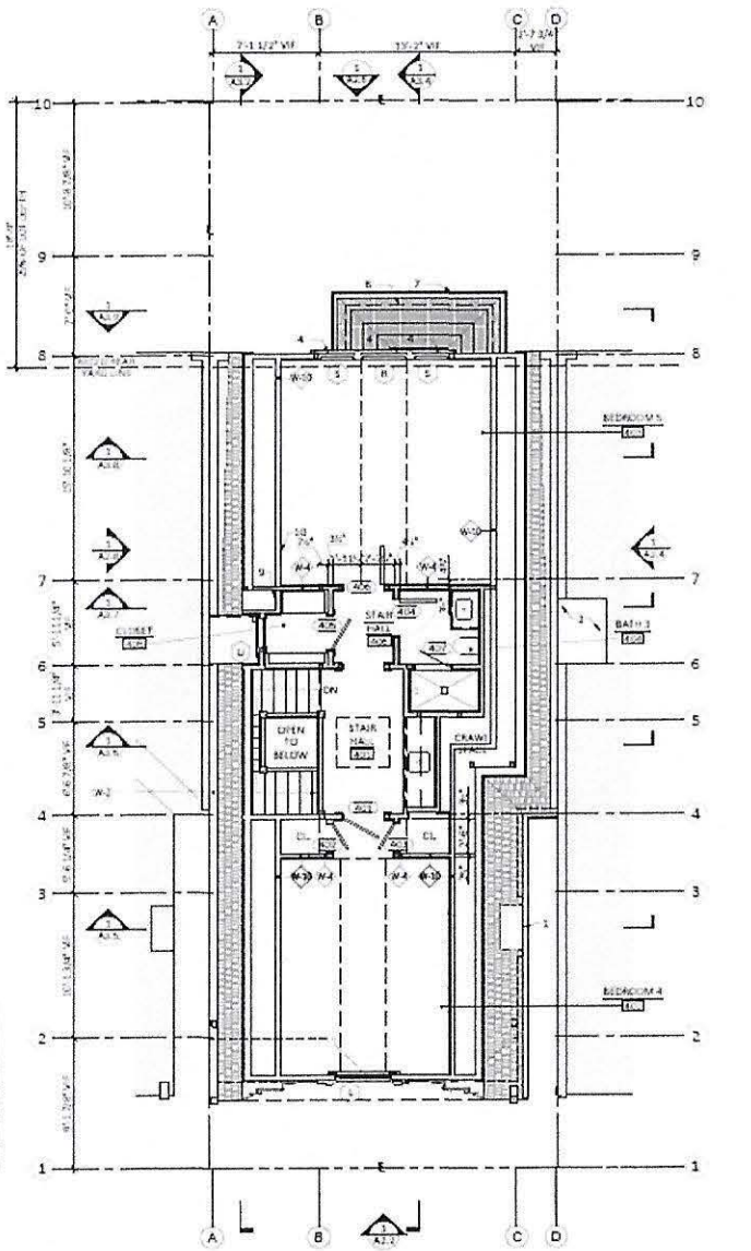
FOURTH FLOOR PLAN - PROPOSED 1/4" = 1'-0"
