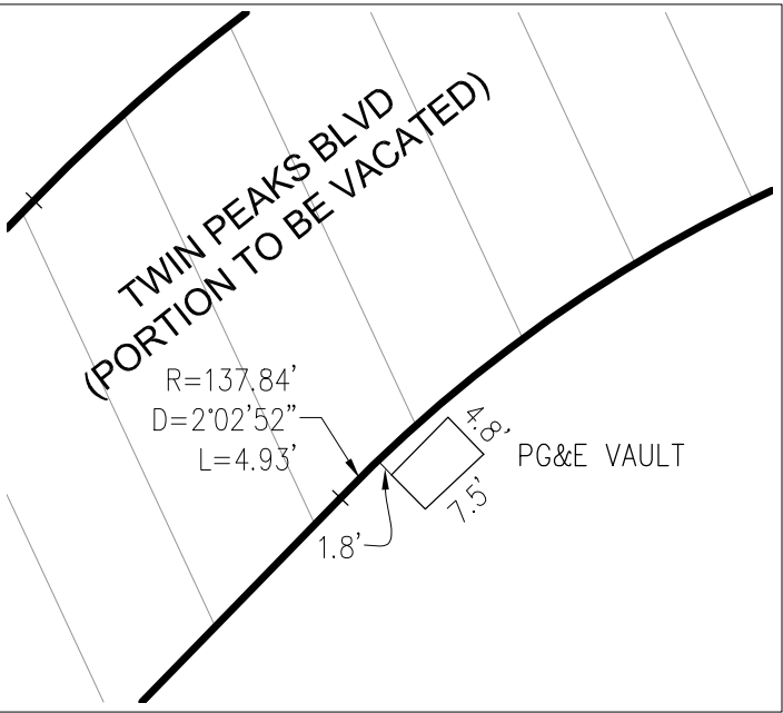
DETAIL E
