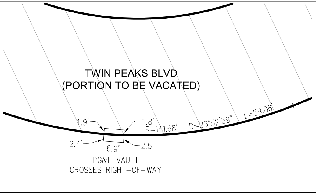
DETAIL D
