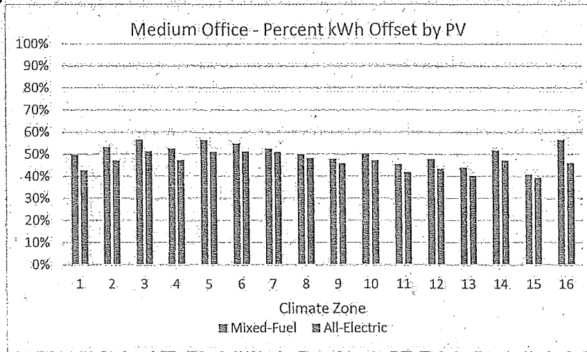
Figure 5. Medium Office – Annual Percent kWh Offset with 135 kW Array
