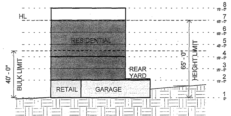
Section 1" = 30'-0"
