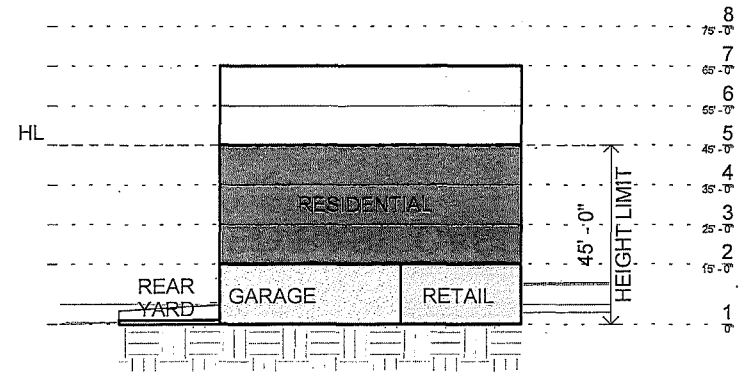
Section 1" = 30'-0"
