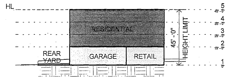
Section 1" = 30'-0"
