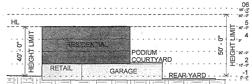
Section 1" = 30'-0"
