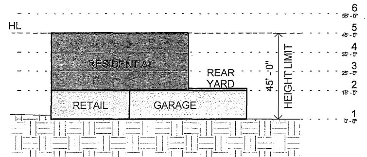
Section 1" = 30'-0"
