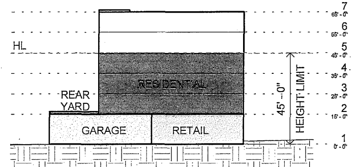
Section 1" = 30'-0"
