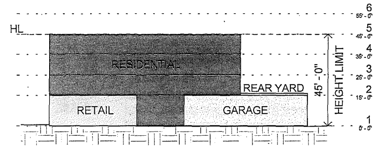
Section 1"=30'-0"
