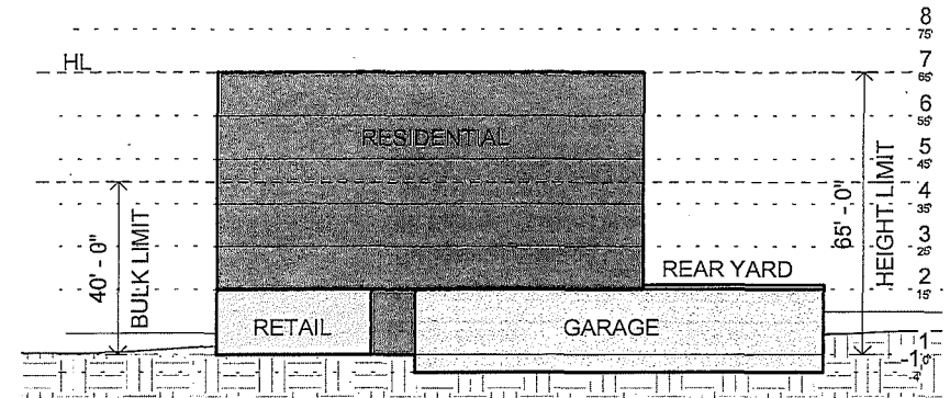
Section 1" = 30'-0"
