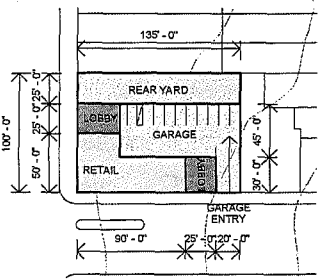
1 1" = 100'-0"
