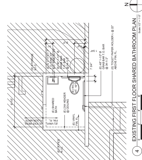
4 EXISTING FIRST FLOOR SHARED BATHROOM PLAN Scale: 1/2" = 1'-0"
