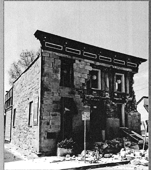
Damaged building in downtown Napa. Photograph by Erol Kalkan, U.S. Geological Survey.
