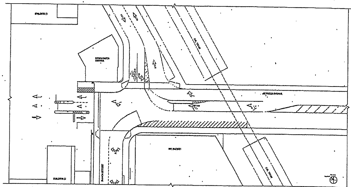
1 - MARKET ST. - EASTERN INTERSECTION 1" = 30'
