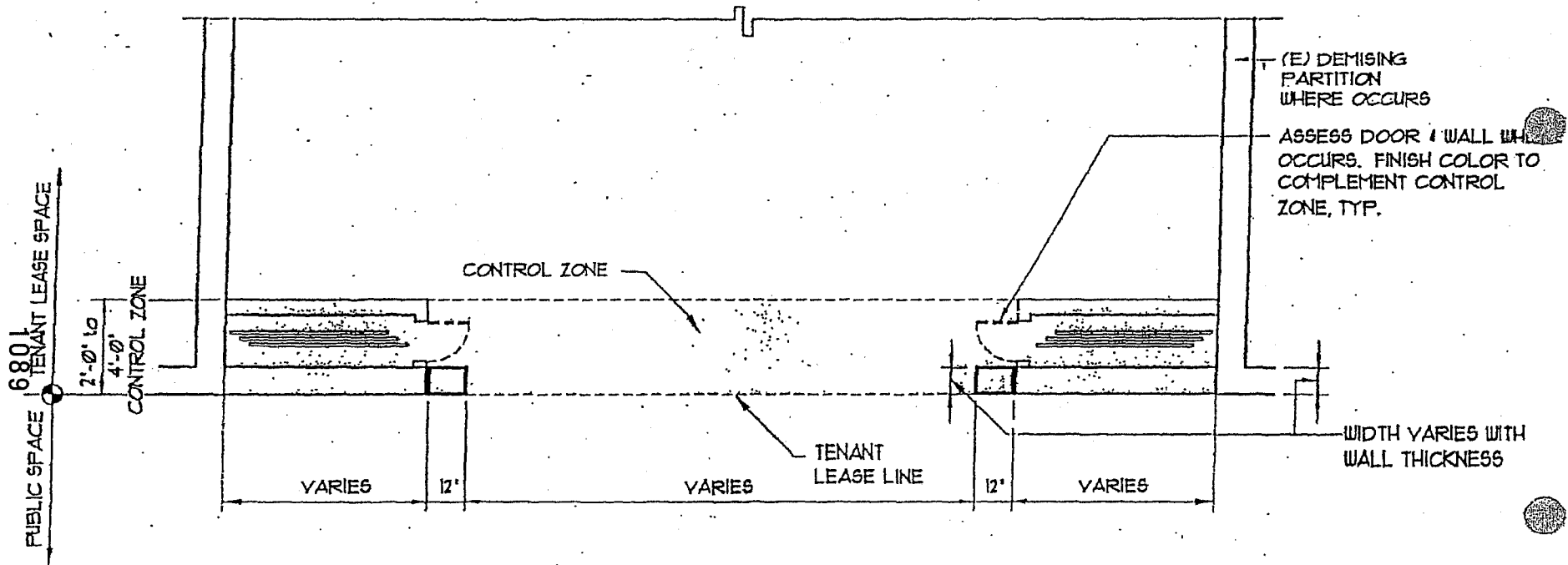
FLOOR PLAN - CONDITION #1
