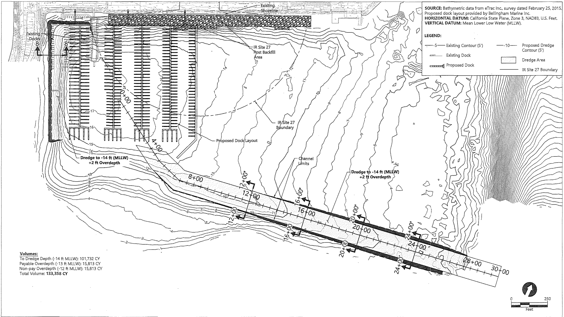
Figure 3 Conceptual Dredging Plan
