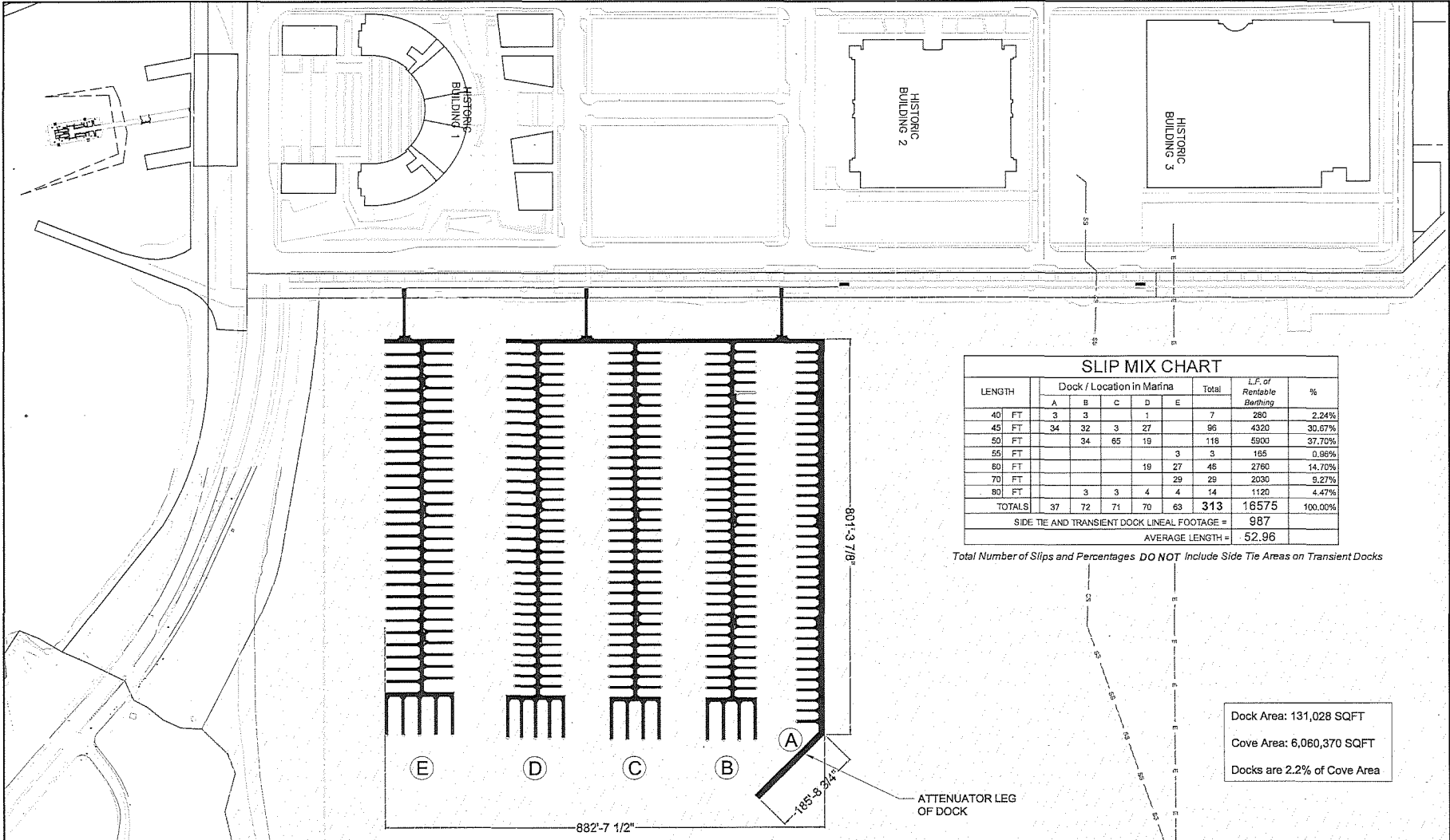
FIGURE 2- Proposed Marina Configuration
