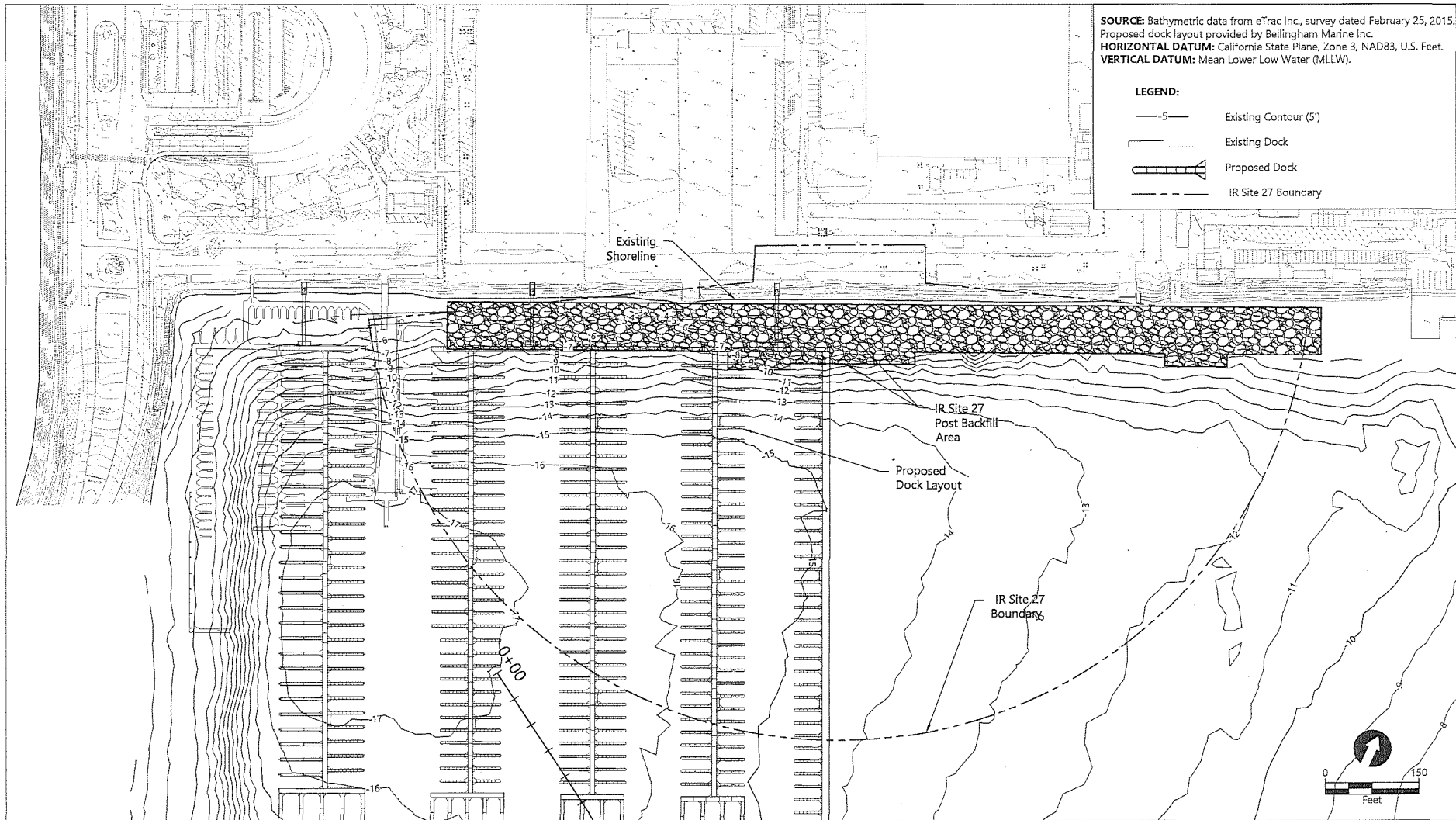
Figure 8 IR Site 27 Conceptual Dredging Treasure Island Marina
