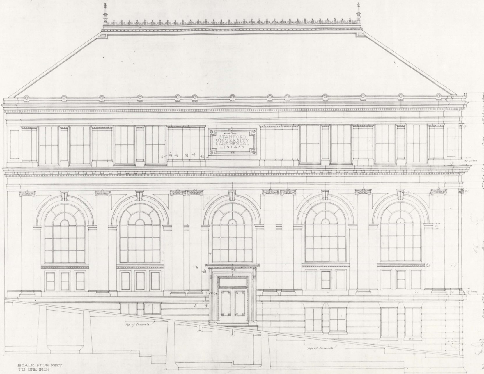
ELEVATION ON SACRAMENTO STREET
