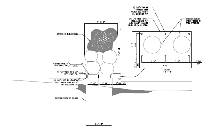
4 ARTWORK 4 ELEVATION 17th & VERMONT ST. 1/8" = 1'-0"
