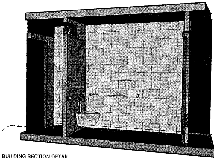
BUILDING SECTION DETAIL
