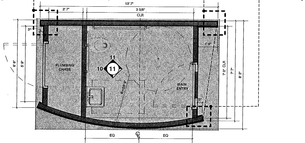
FLOOR PLAN - SINGLE OCCUPANCY - BASIC MODULE
