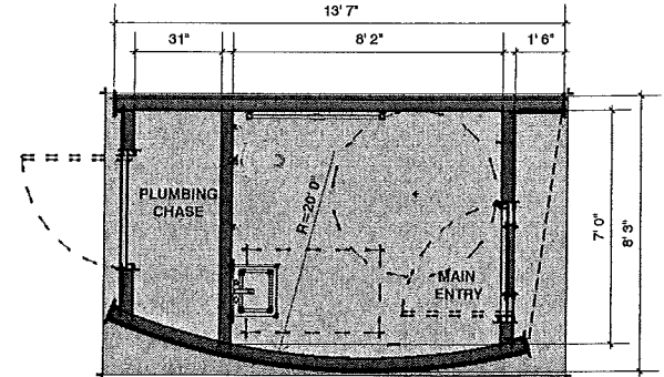
FLOOR PLAN - SINGLE OCCUPANCY - BASIC MODULE
