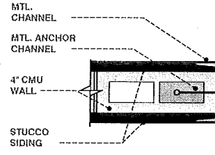
WALL DETAIL 2
