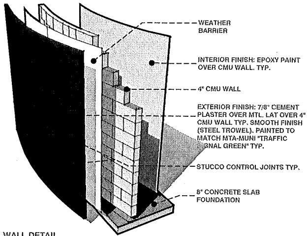
WALL DETAIL
