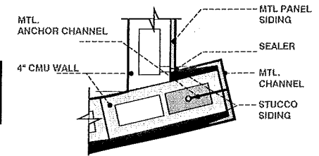
WALL DETAIL 3
