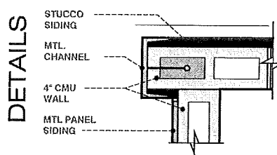
WALL DETAIL 1
