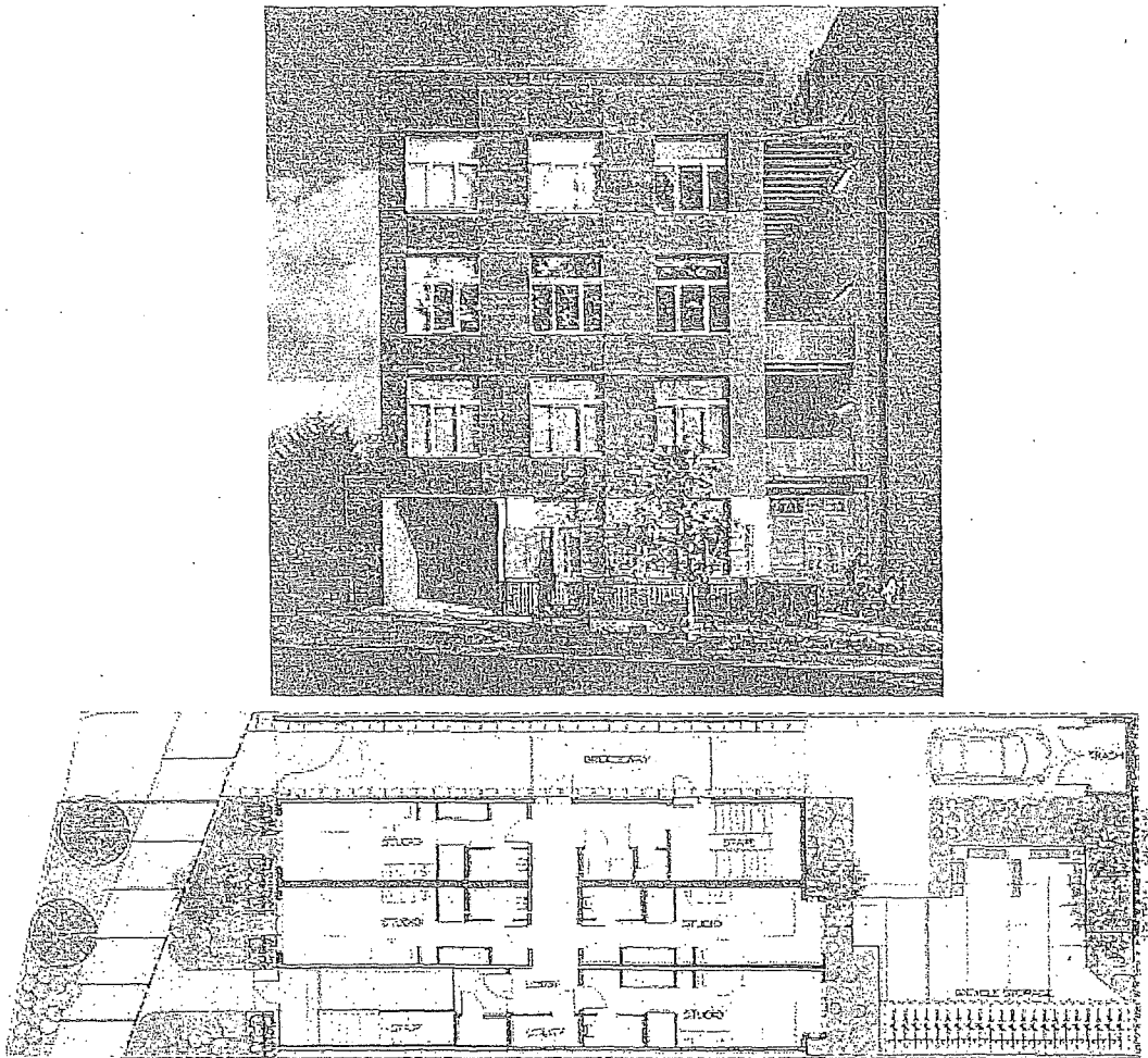
Figure 6: 2711 Shattuck Façade and Ground Floor Site Plan
