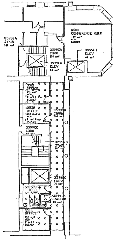
5TH FLOOR
