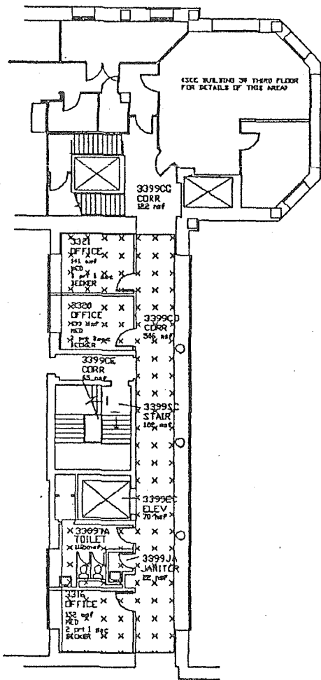
3RD FLOOR
