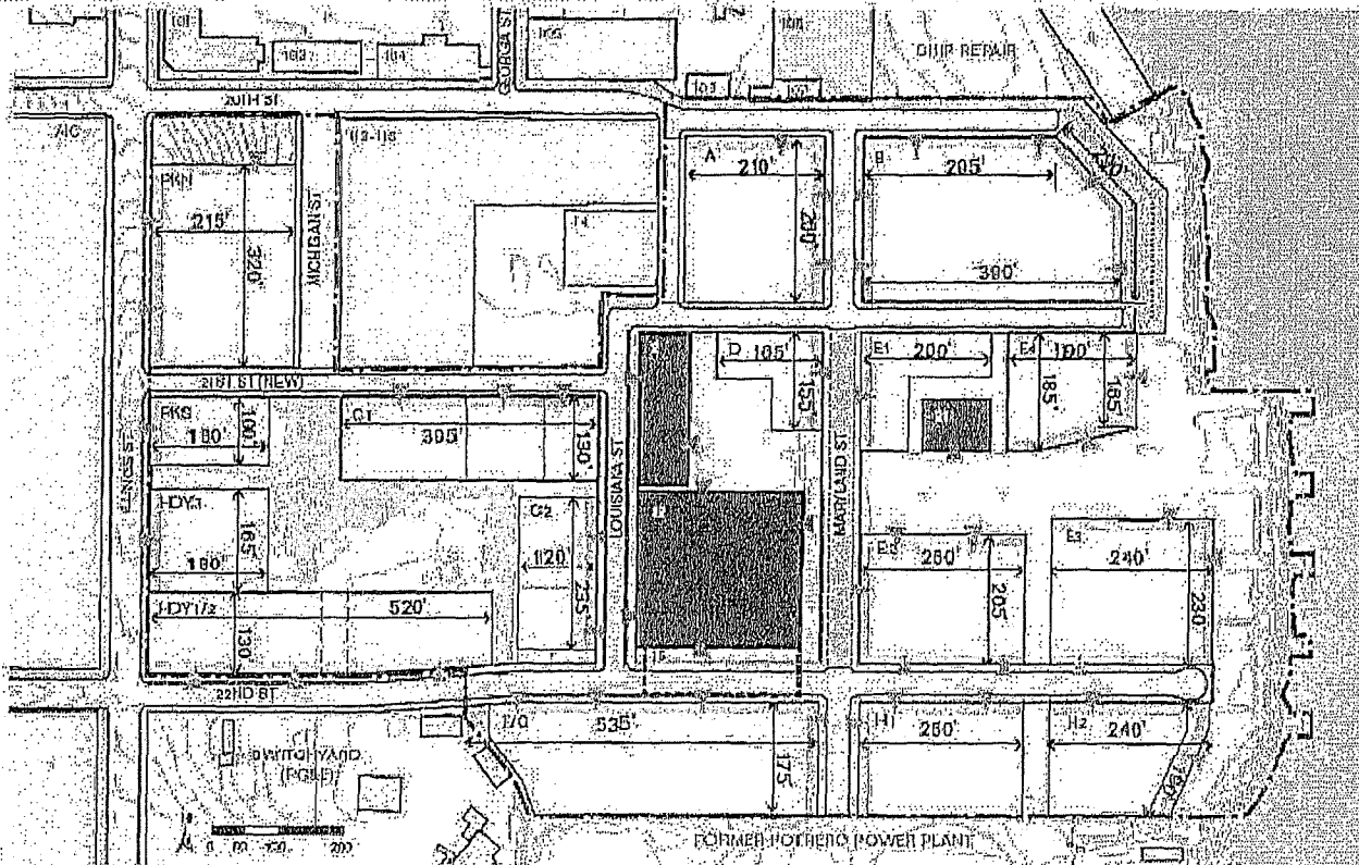
FIGURE 6.8.5: Illustrative Plan of Building Entries from Public Right of Way Note: All dimensions are rounded up to the nearest 5'
