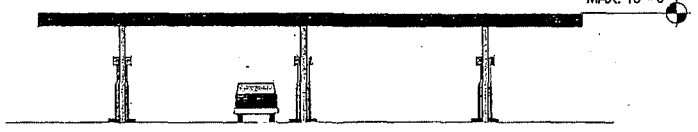
④ ELEVATION - CCSF FUEL STATION FRONT 1/16" = 1'-0"
