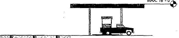
⑤ ELEVATION - CCSF FUEL STATION SIDE 1/16" = 1'-0"
