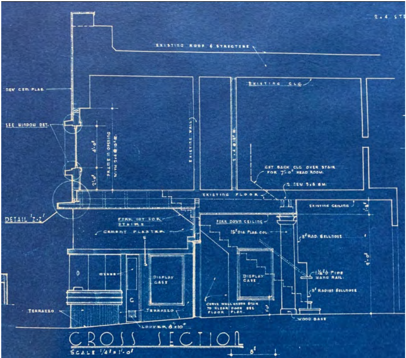
Architect Vincent G. Raney, Section Drawing, 1946 Source: Gary Parks Collection, posted on San Francisco Theatres: Clay Theatre website at http://sanfranciscotheatres.blogspot.com/search/label/Clay%20Theatre
