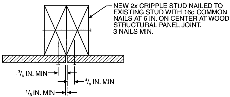
VERTICAL SPLICE AT DOUBLE STUD
