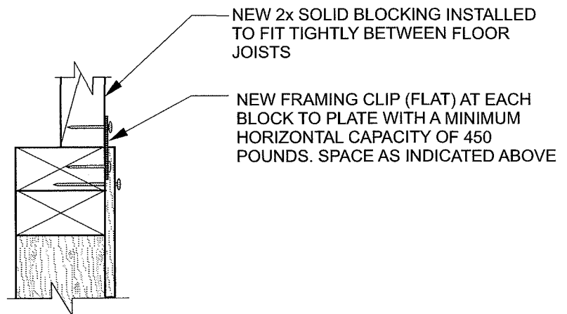
ALTERNATE DETAIL FOR FLUSH CONDITION
