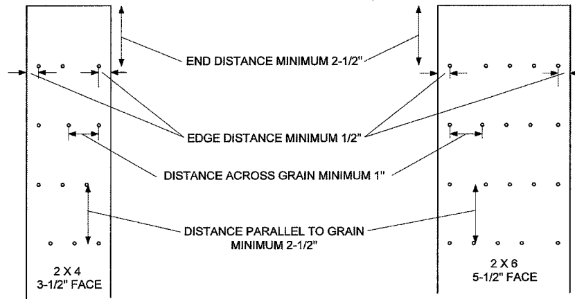
[BS] FIGURE C103.6.3 FASTENER SPACINGS FOR LUMBER-TO-LUMBER CONNECTIONS OPERATING IN SHEAR PARALLEL TO GRAIN
