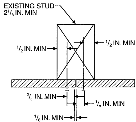
VERTICAL SPLICE AT SINGLE STUD
