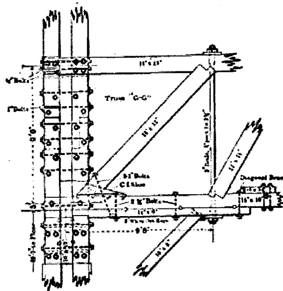
FIG. 6d.—Howe Truss, Horticultural Building, Pan-American Exposition.
