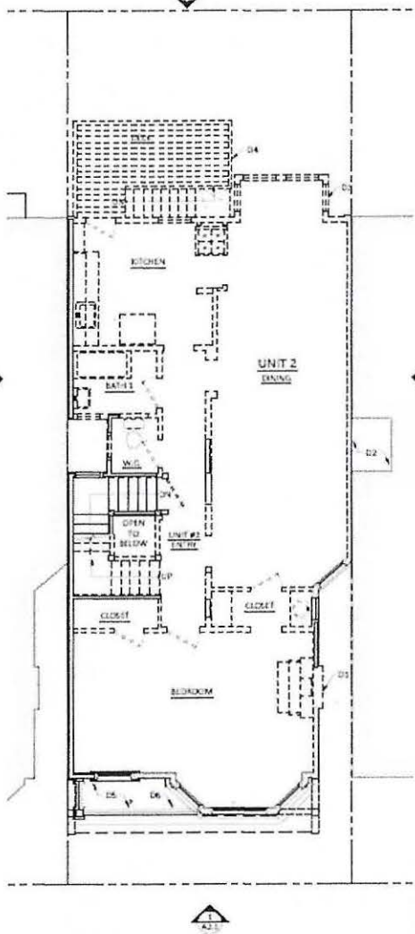
THIRD FLOOR PLAN - EXISTING AND DEMOLITION 1/4" = 1'-0" 2
