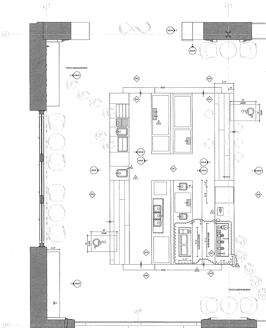
1 ENLARGED PLAN - LEVEL 03 - COFFEE BAR SCALE: 1/8" = 1'-0"
