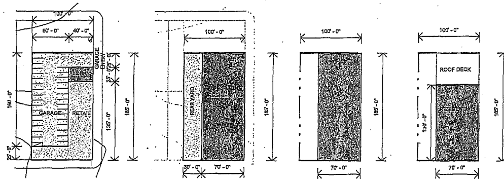
1 1"=100'-0" 2 1"=100'-0" 3 1"=100'-0" 4 1"=100'-0"
