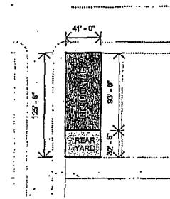
2 1" = 100'-0"
