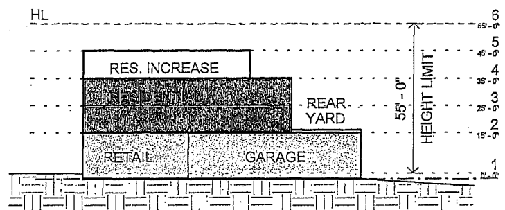
Section 1" = 30'-0"
