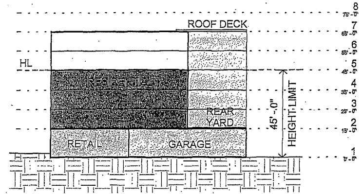
Section 1" = 30'-0"
