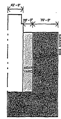
2 1"=100'-0"
