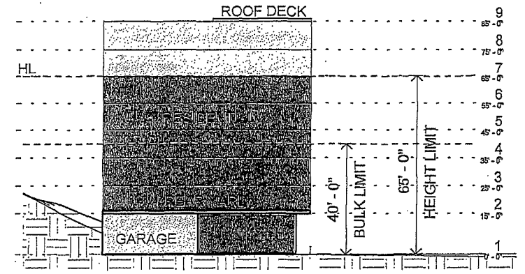
Section 1" = 30'-0"
