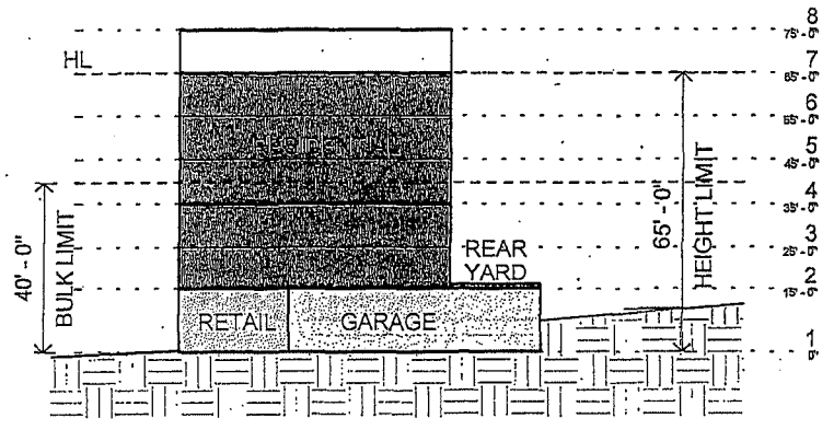
Section 1" = 30'-0"
