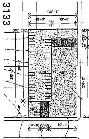
1 1" = 100'-0"
