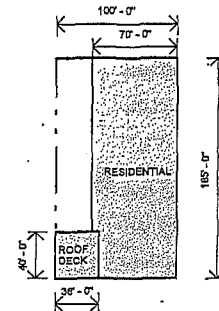
7 1" = 100'-0"
