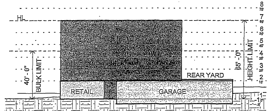
Section 1" = 30'-0"
