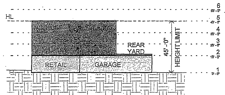
Section 1"=30'-0"
