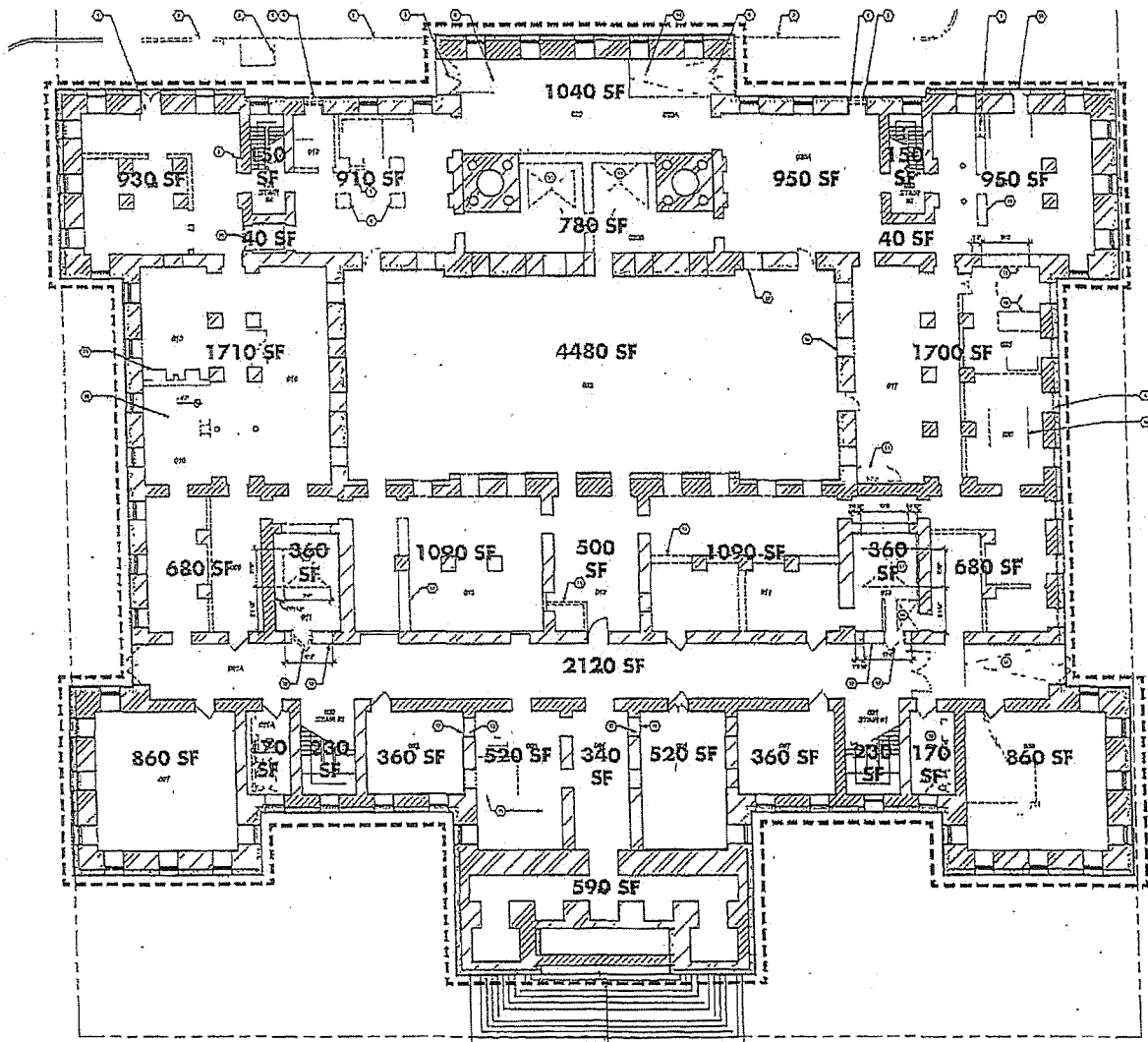
GROUND FLOOR PLAN with areas
