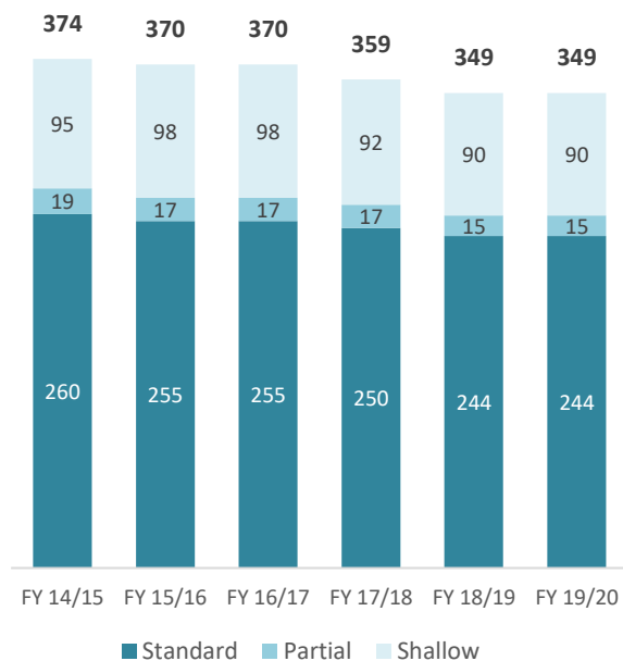
Figure 4: SFAF Subsidies by Type, FY 14/15 to FY 19/20
