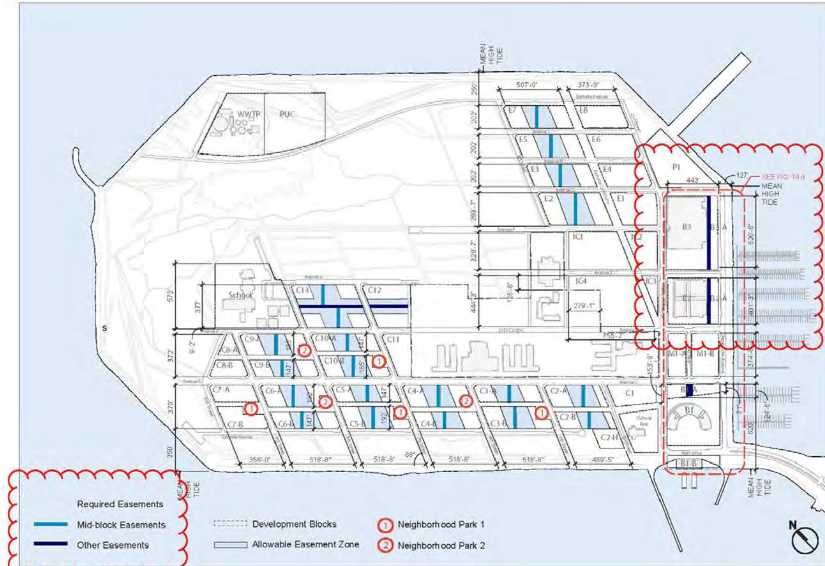
Figure 14.c. Development Block and Easement Plan (Dimensions subject to change at Final Tentative Map)
