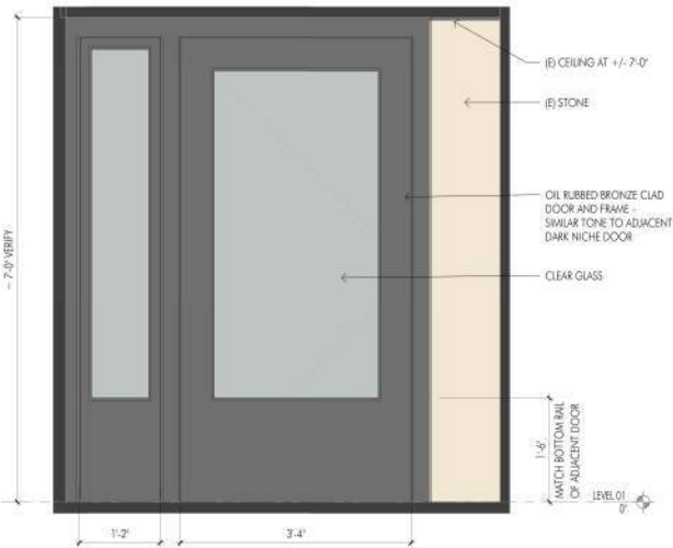
2 PROPOSED ELEVATION LOBBY SIDE DOORS 1" = 1'-0"
