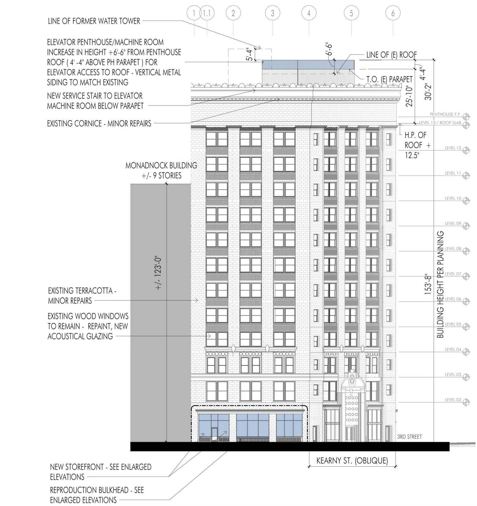
PROPOSED MARKET STREET ELEVATION
