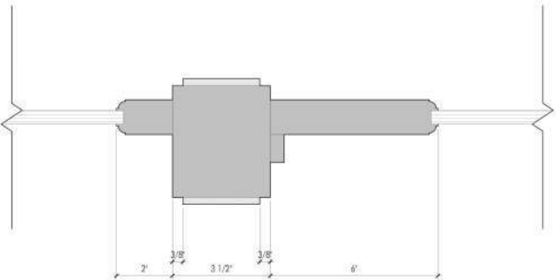
3 PROPOSED LOBBY DOOR TO SIDELITE JAMB 6" = 1'-0"
