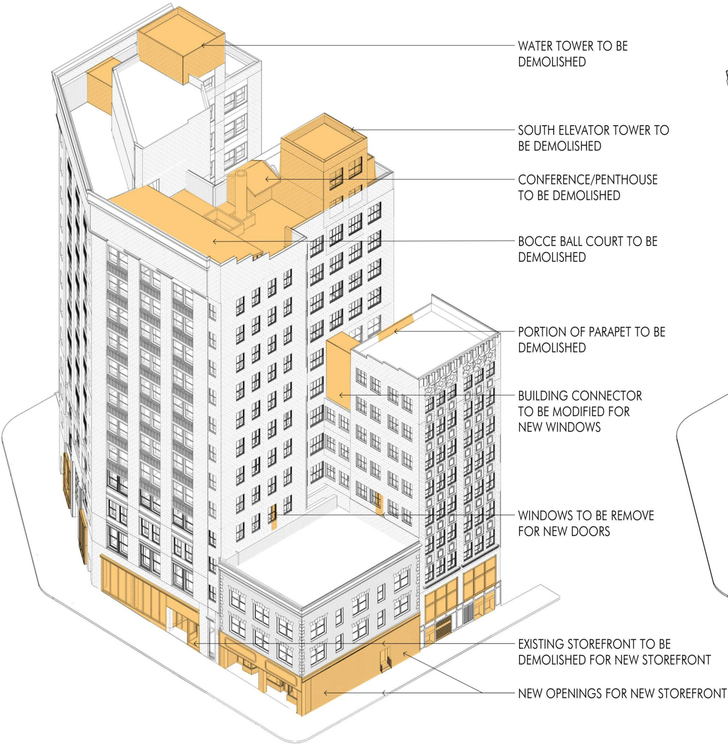
1 EXISTING HEARST BUILDING 1/2" = 1'-0"
