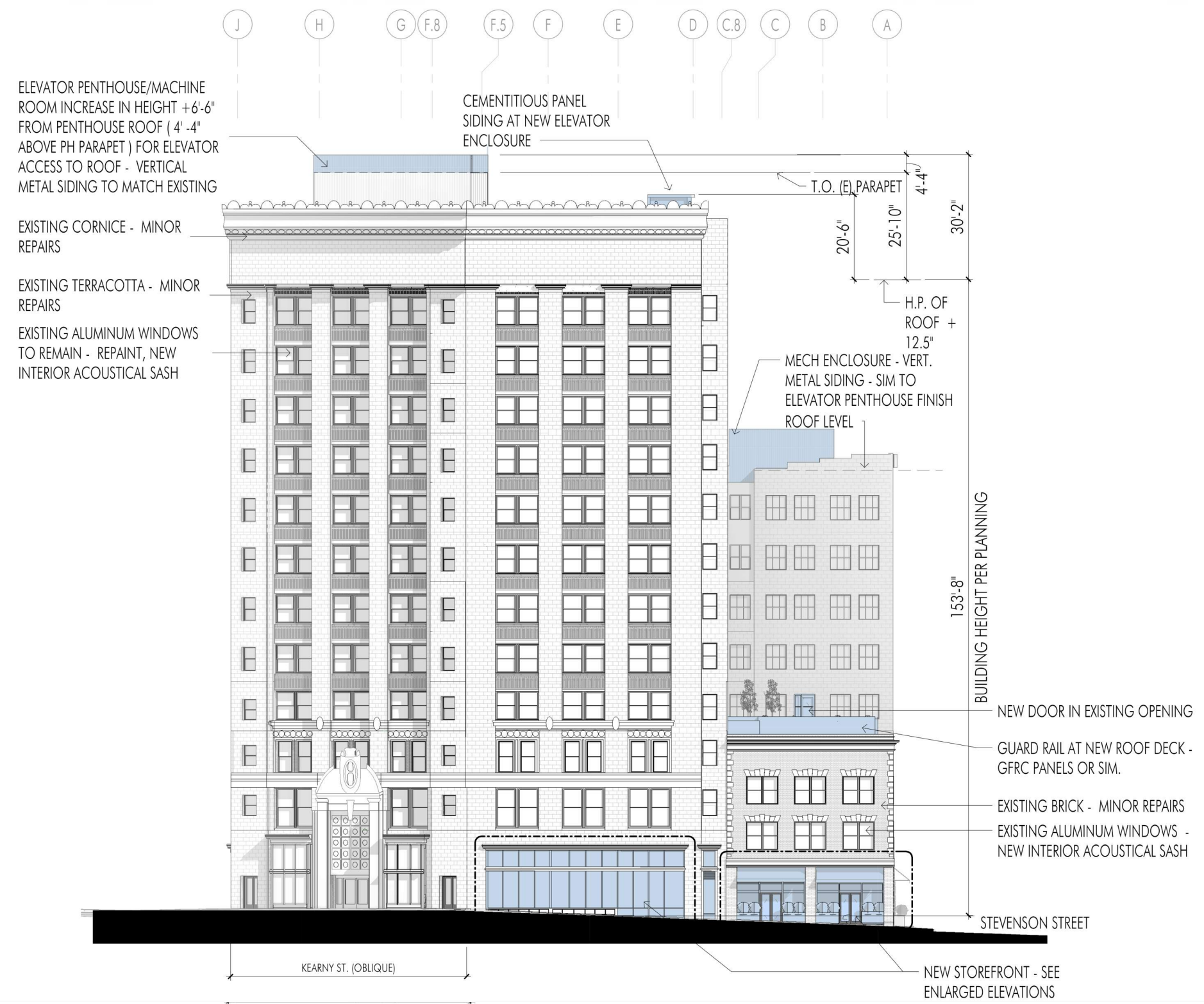
PROPOSED THIRD STREET ELEVATION
