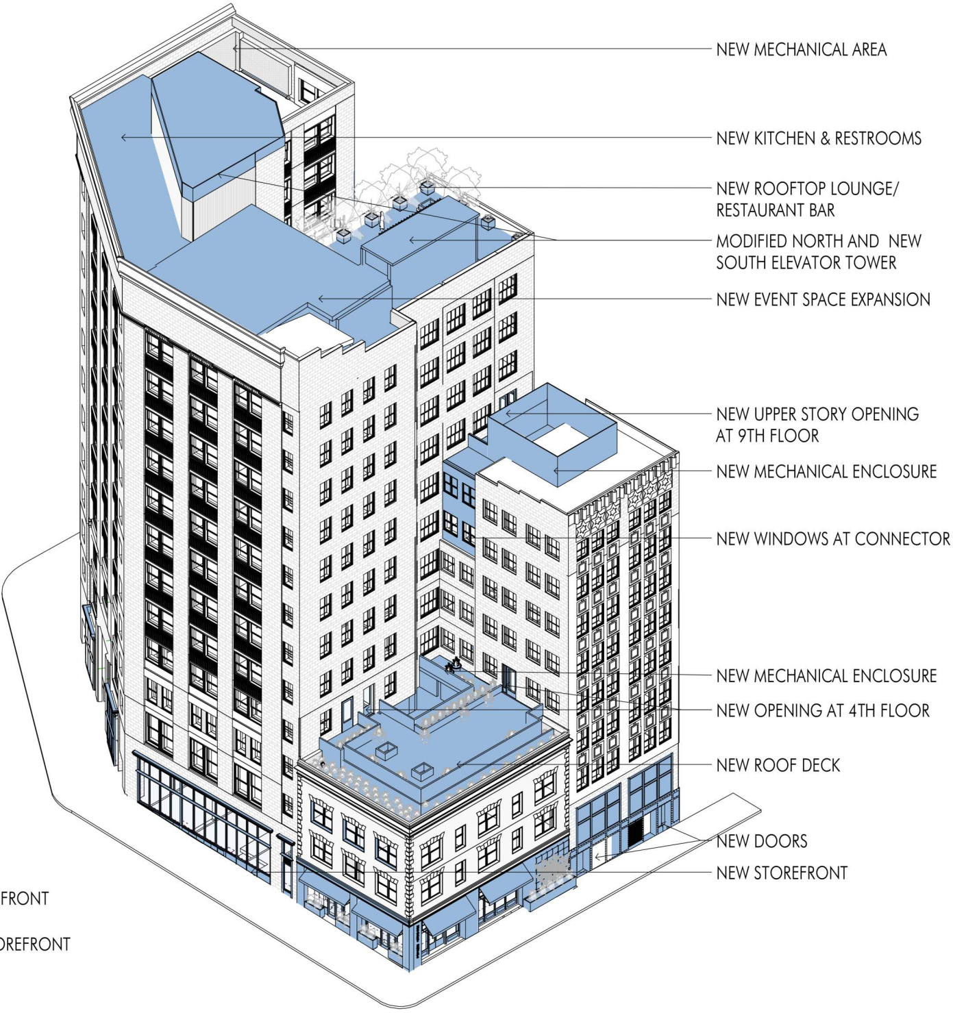
2 PROPOSED HEARST BUILDING 1/2" = 1'-0"
