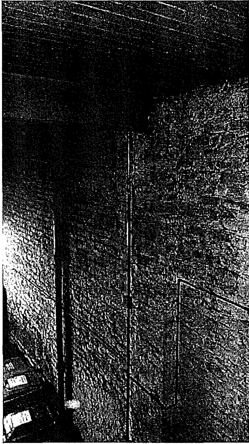
Figure 15 Steel frame visible at the utility area at the east end of the building. Note the I-beam and brick-veneer pilaster containing the steel column at the intersection of the northern and central structural bays. View of the east wall, photographed to the northeast.
