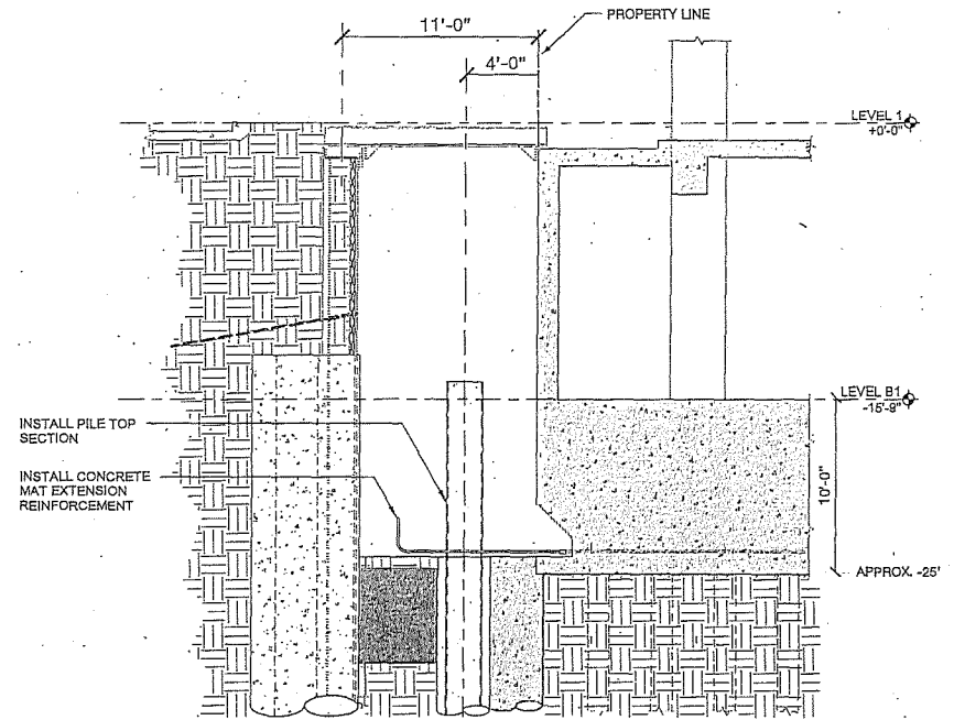
STEP 9 INSTALL CONCRETE MAT EXTENSION REINFORCEMENT AND PILE TOP SECTION
