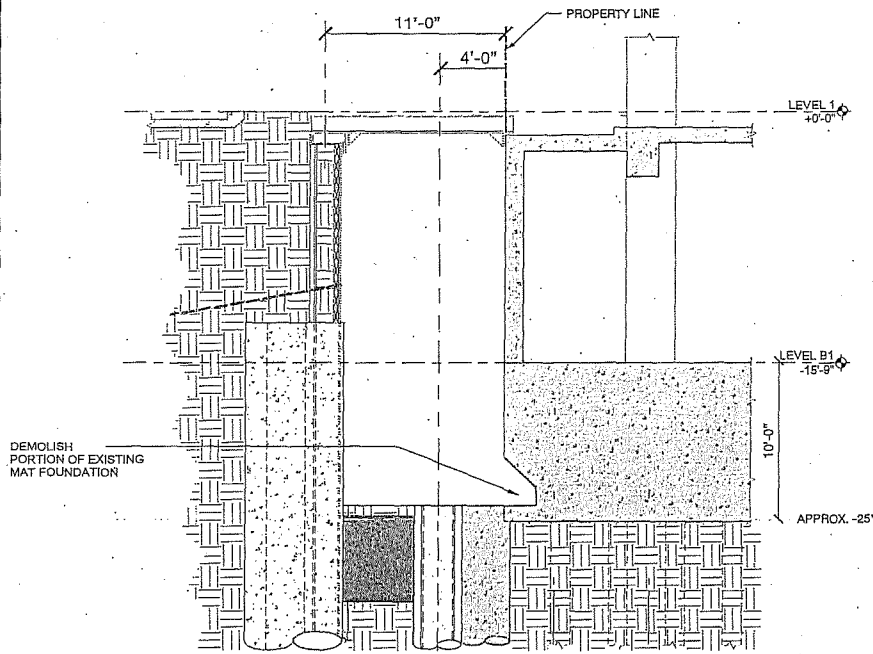
STEP 8 EXCAVATE TO BOTTOM OF MAT
