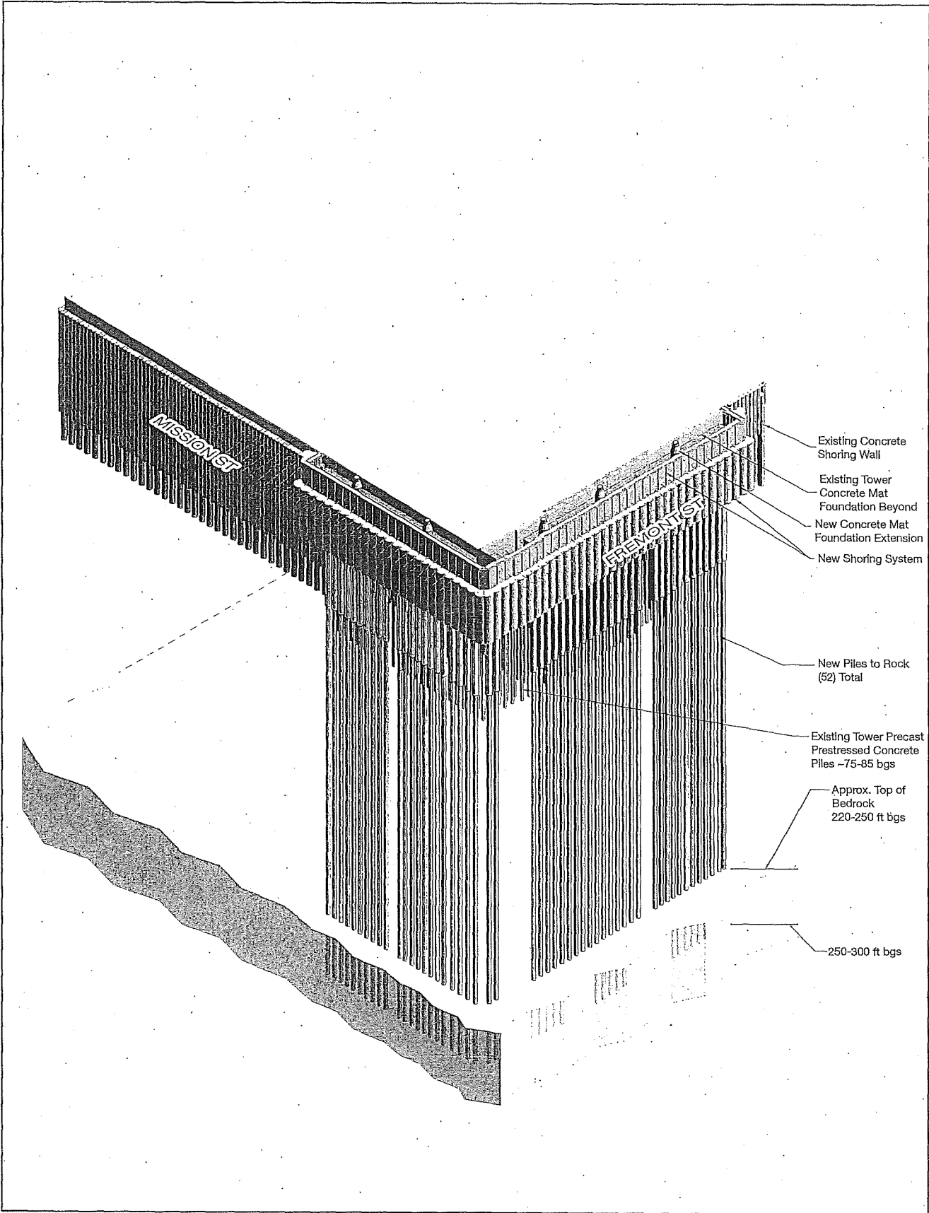
Figure 4 Current and Proposed Foundation System (Looking Southeast)
