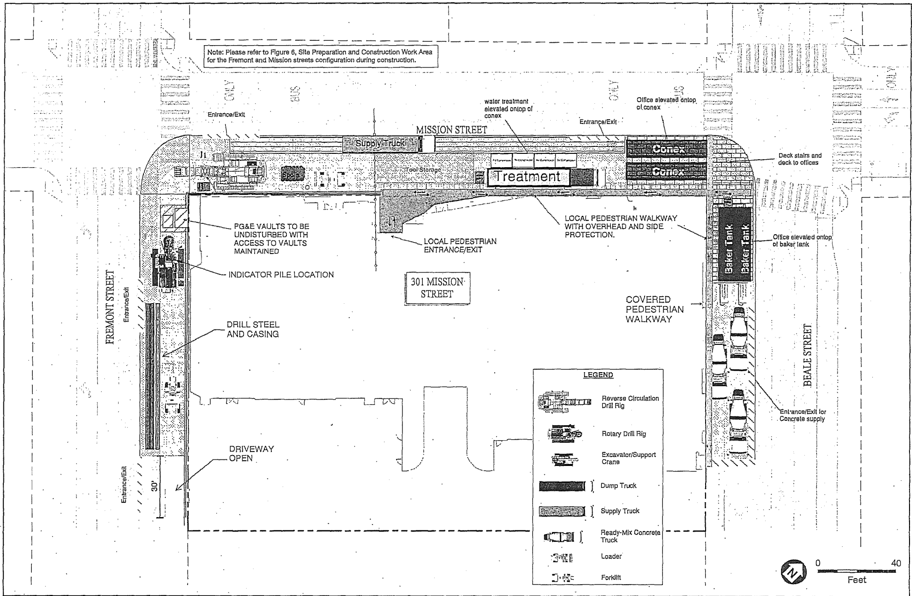
Figure 7 Stage 1: Mobilization and Indicator Pile
