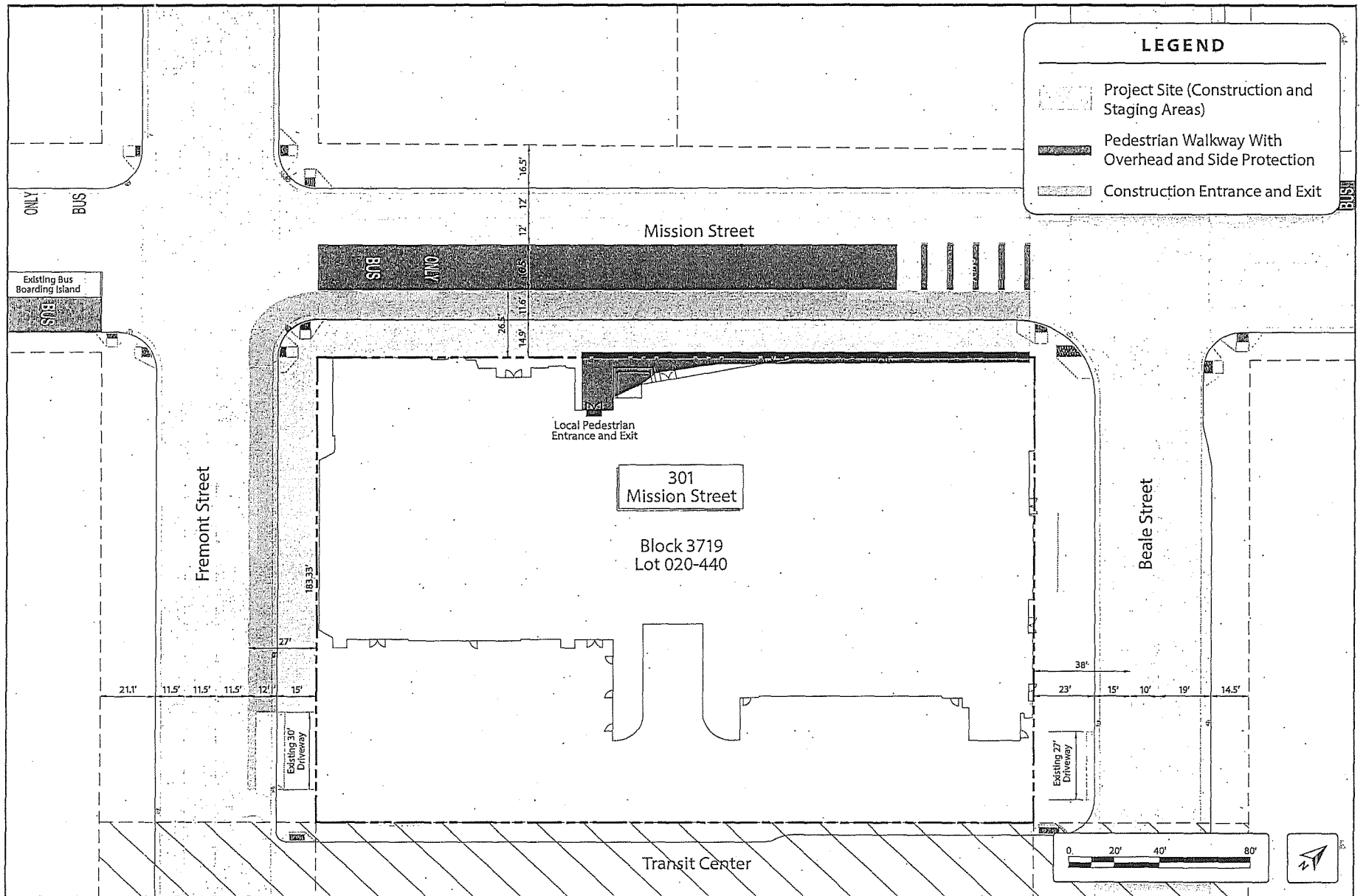
Figure 26 Construction Boundary During Stage 6
