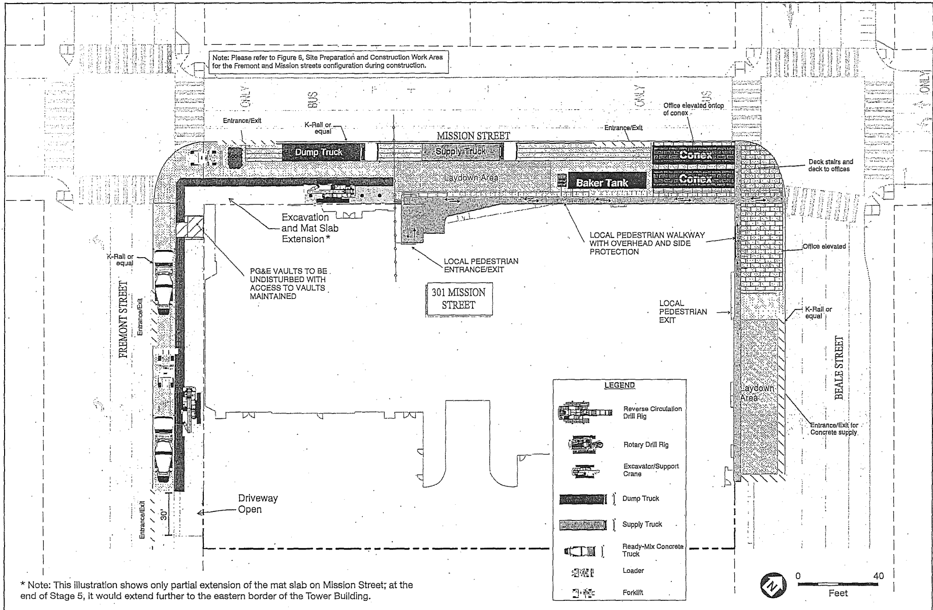
Figure 16 Stage 5: Mat Slab Extension on Mission Street
