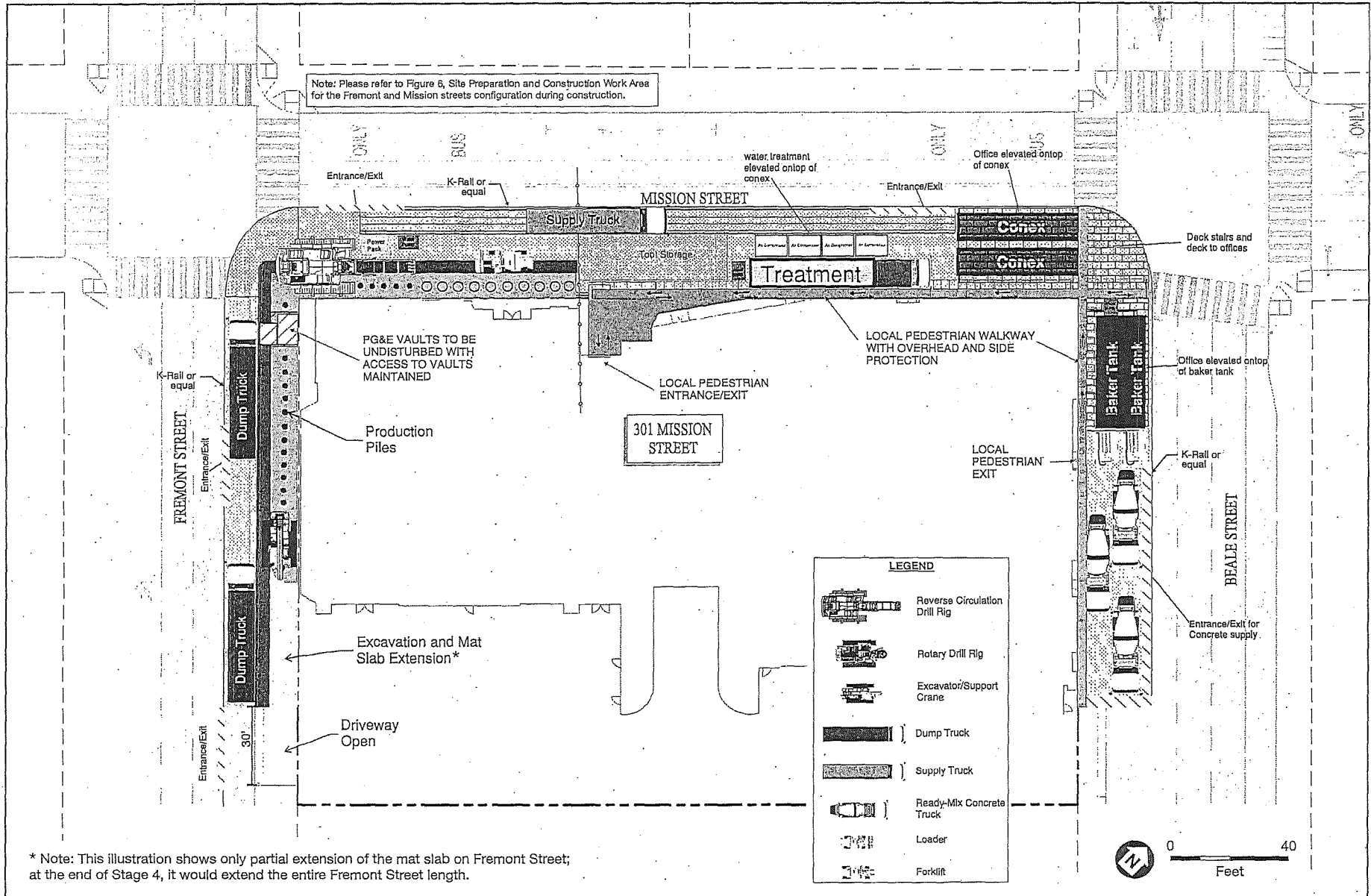
Figure 13 Stage 4: Piles on Mission Street and Construction of Mat Slab Extension on Fremont Street
