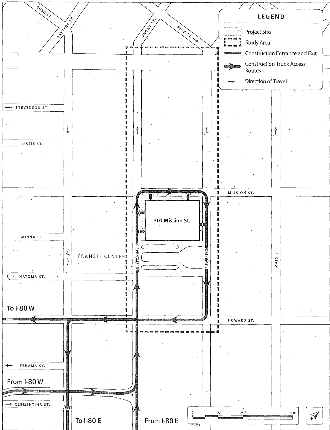
Figure 24 Construction Truck Access Routes
