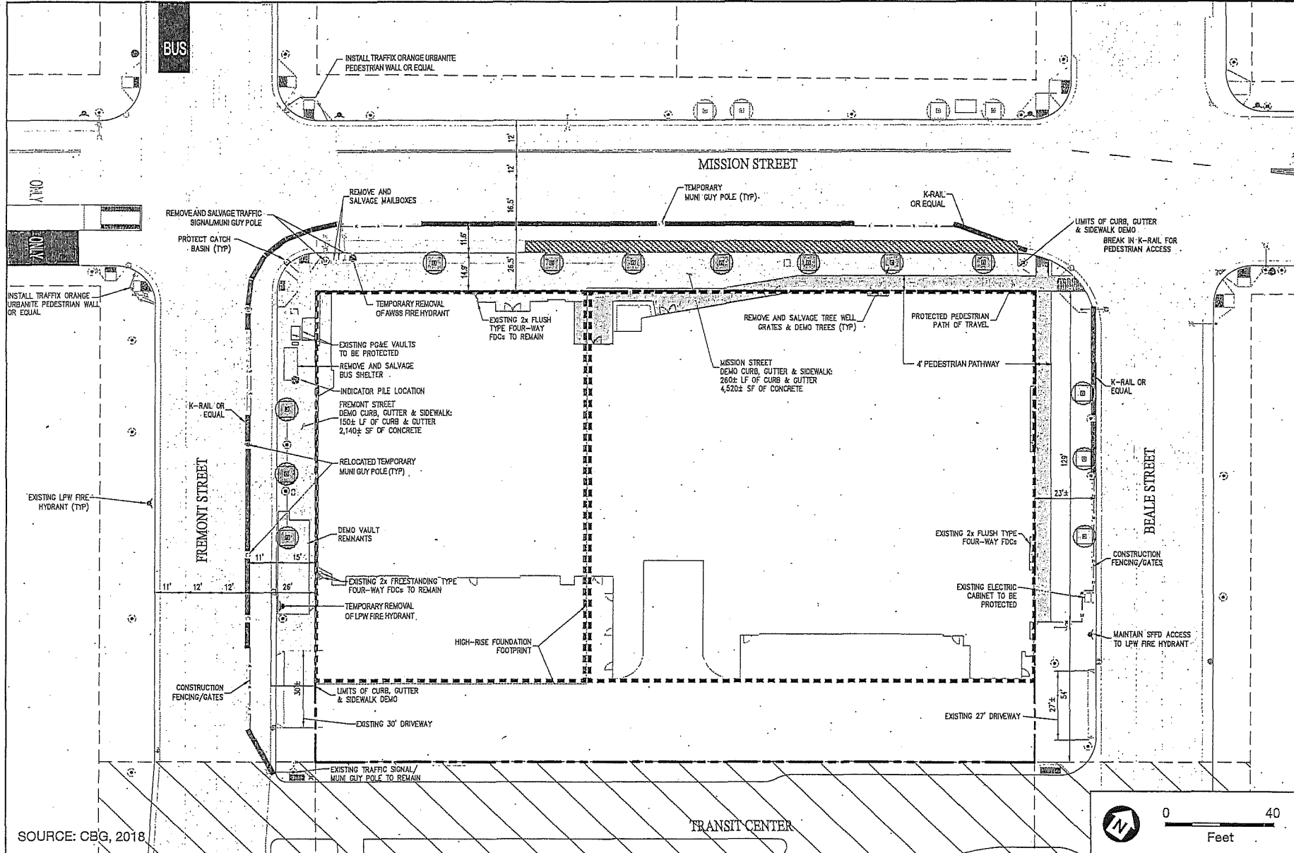
Figure 6 Stage 1: Site Preparation and Construction Work Area
