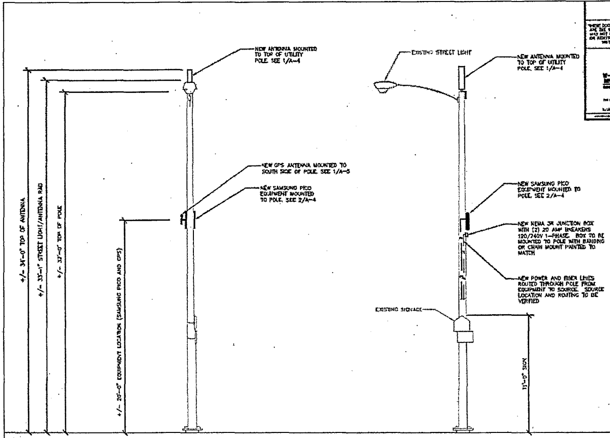
Exhibit 1: Sample Street Light with DAS Equipment Design
