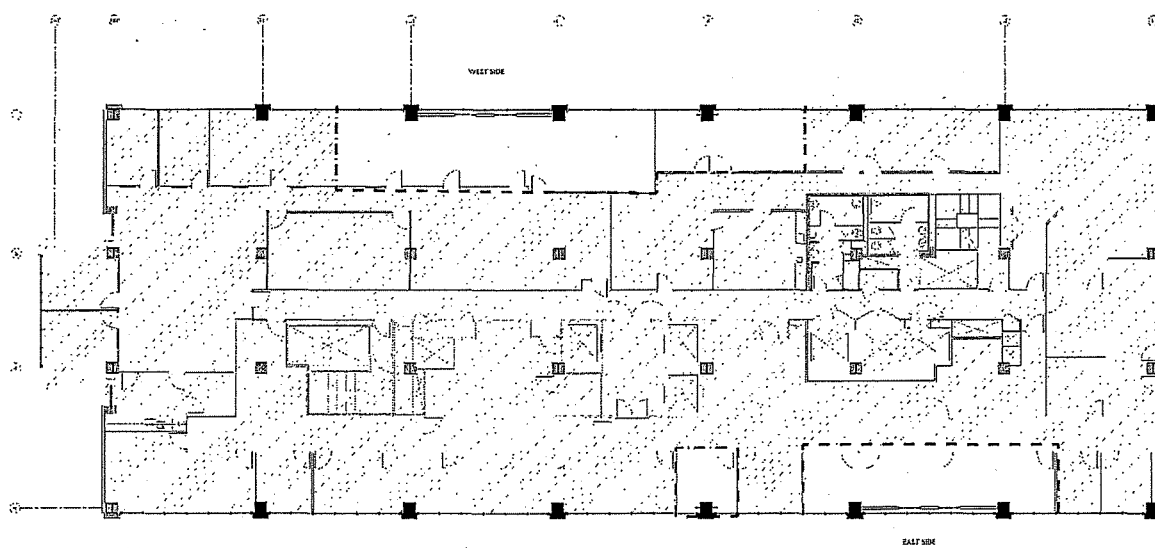
FOURTH FLOOR CONST. PLAN A2.06
