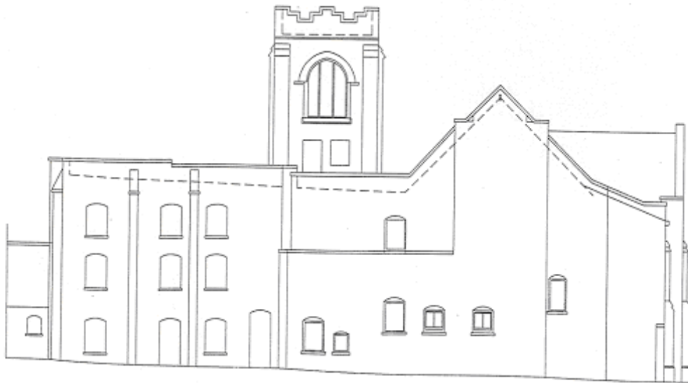
EAST ELEVATION
