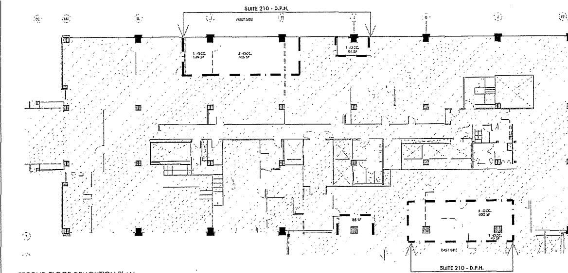
SECOND FLOOR DEMOLITION PLAN
