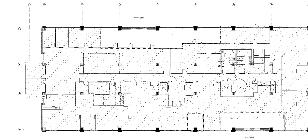
13 FOURTH FLOOR CONST. PLAN SCALE: 1/4" = 1'-0"
