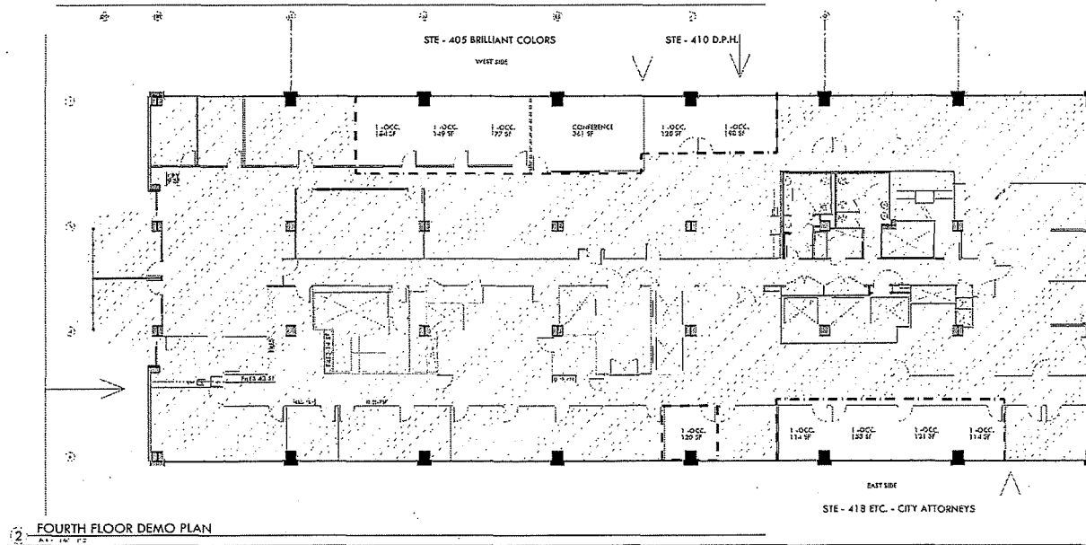
12 FOURTH FLOOR DEMO PLAN SCALE: 1/4" = 1'-0"
