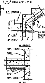
7 TYPICAL SLAB-ON-GRADE DETAILS SCALE 3/4" = 1'-0"
