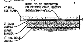
7 TYPICAL SLAB-ON-GRADE DETAILS SCALE 3/4" = 1'-0"
