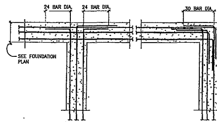
3 TYPICAL GRADE BEAM INTERSECTIONS SCALE 3/4" = 1'-0"
