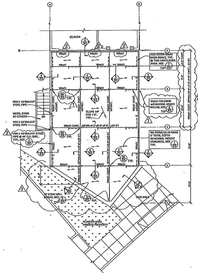
BRIDGE DRIVEWAY FRAMING PLAN SCALE: 1/4"=1'-0"
