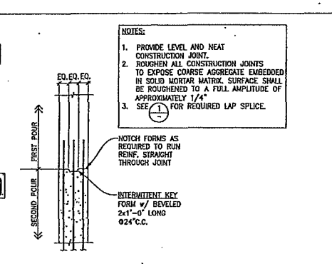
11 TYPICAL CONCRETE WALL CONSTRUCTION JOINT SCALE 3/4" = 1'-0"
