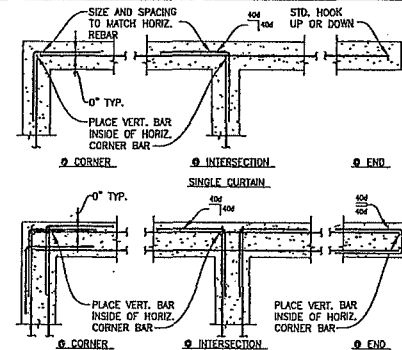
10 CONCRETE WALL INTERSECTION SCALE 1 1/2" = 1'-0"
