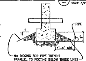
6 PIPE CLEARANCE AND DETAILS @ FOOTING SCALE 3/4" = 1'-0"
