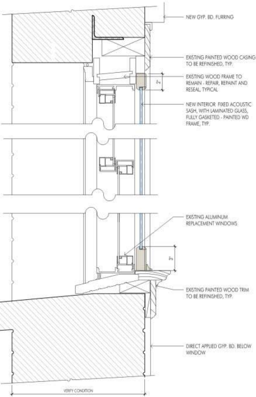
VERTICAL SECTION/ HEAD & SILL
