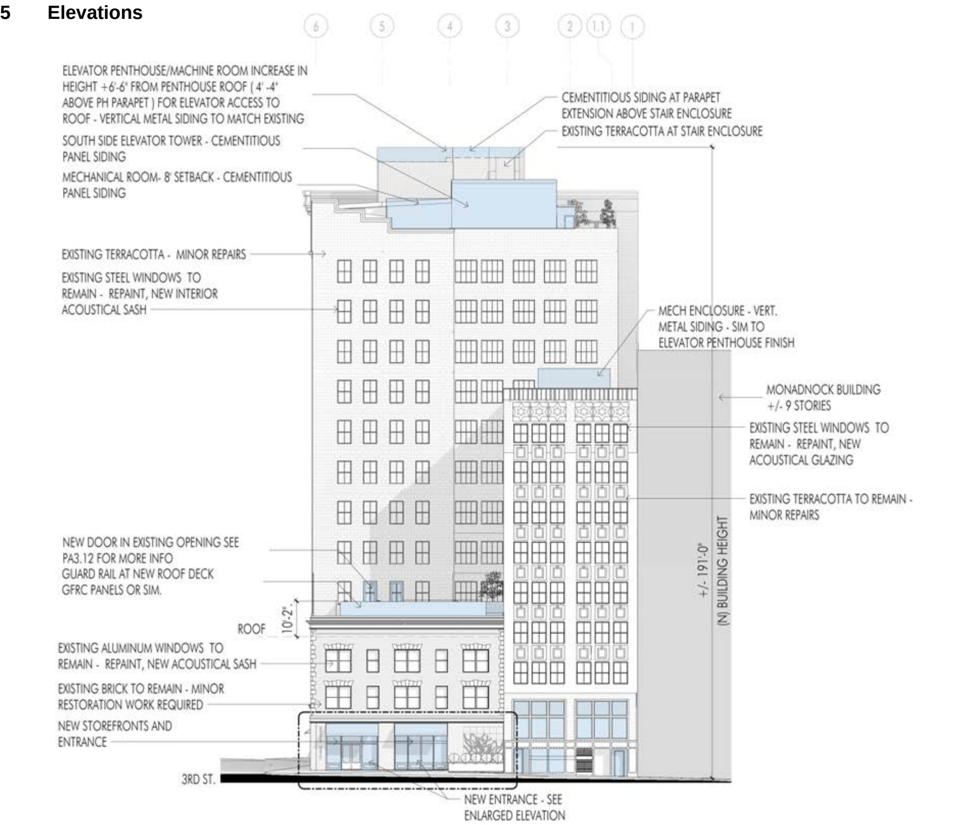
PROPOSED STEVENSON STREET ELEVATION
