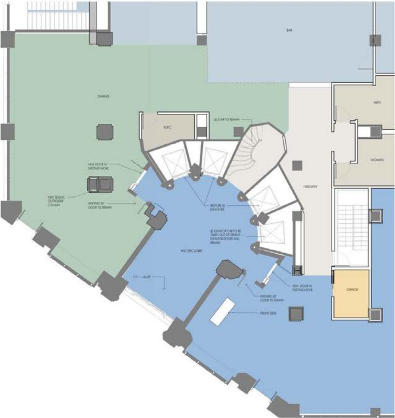
1 ENLARGED LOBBY PLAN 1/16
