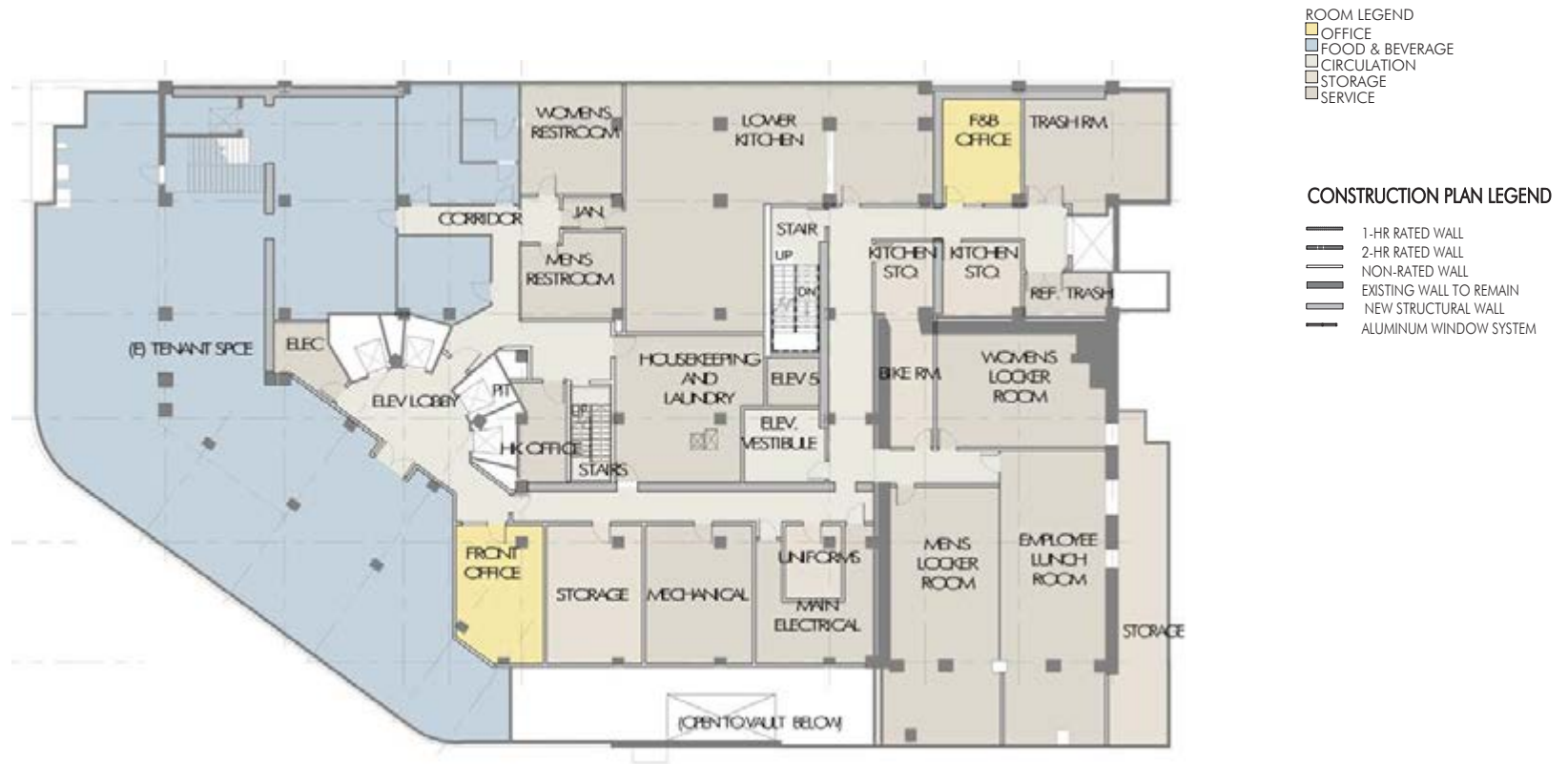
① BASEMENT PLAN
