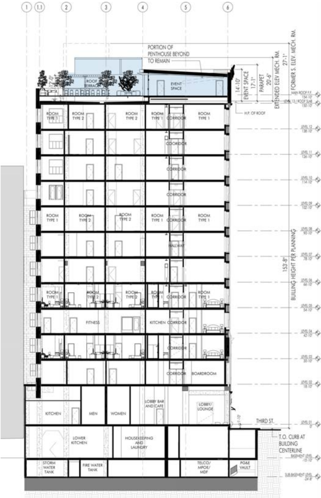
PROPOSED SECTION AT CENTERLINE OF 3 RD STREET looking SOUTH
