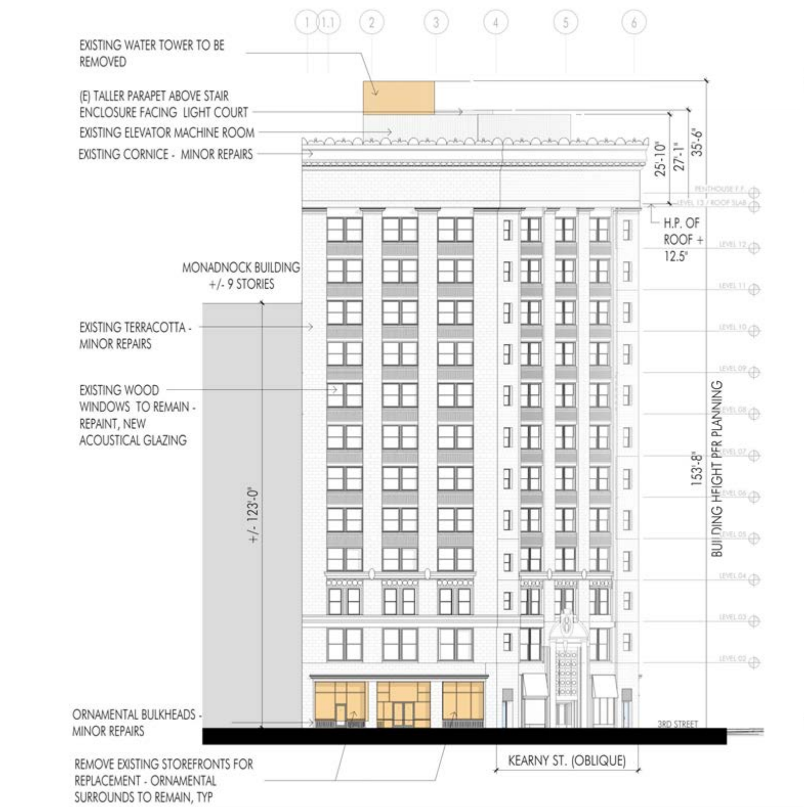
EXISTING MARKET STREET ELEVATION
