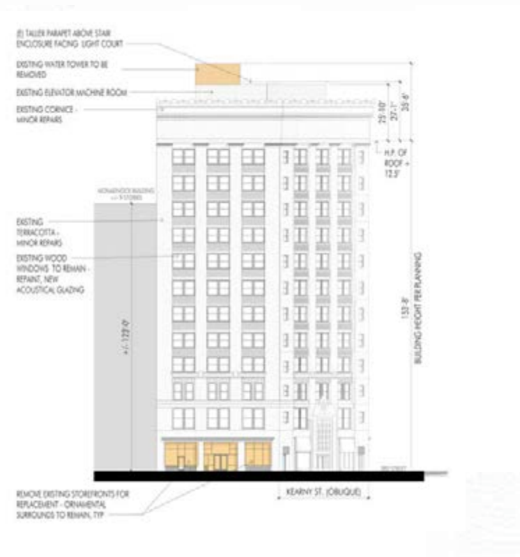
① EXISTING MARKET STREET ELEVATION
