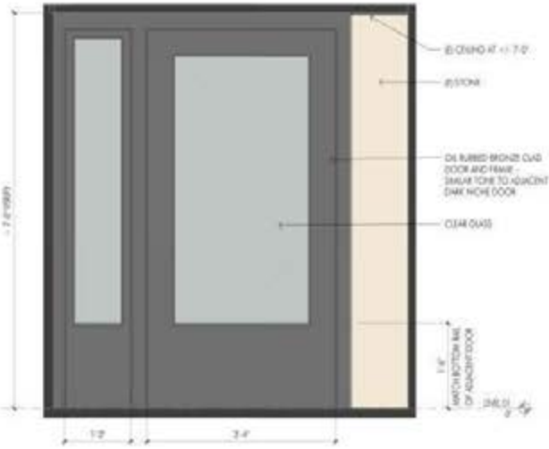
2 PROPOSED ELEVATION LOBBY SIDE DOORS 1/16
