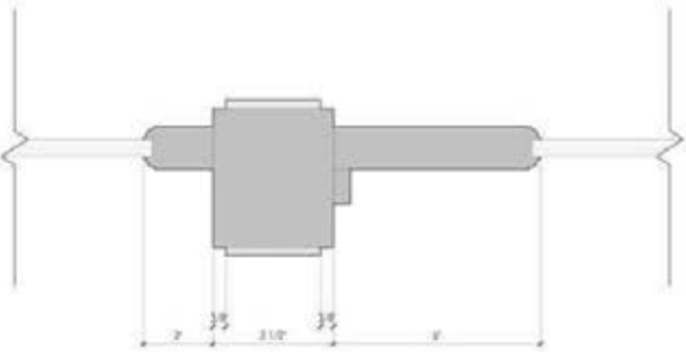
3 PROPOSED LOBBY DOOR TO SIDELITE JAMB 1/16
