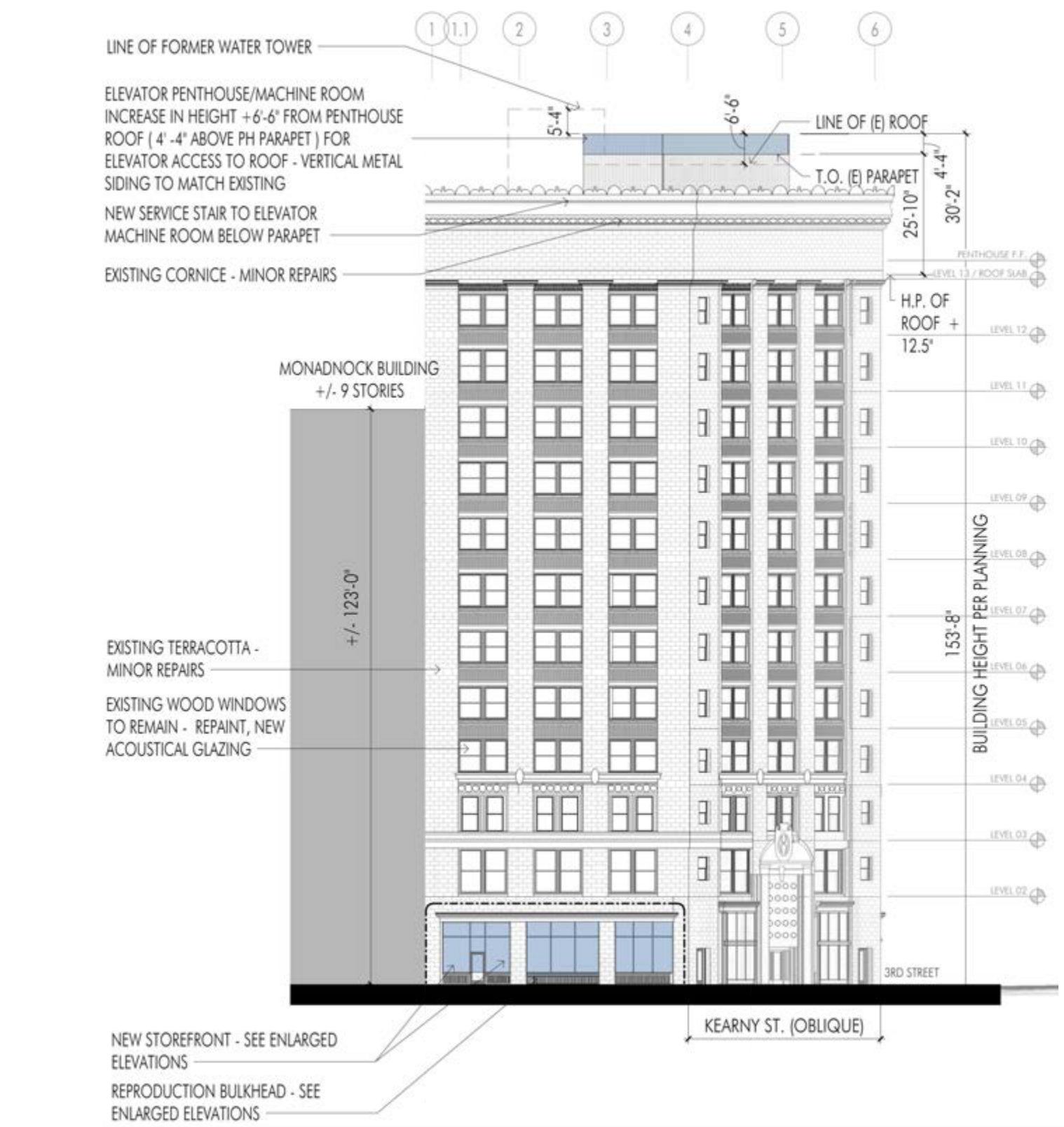
PROPOSED MARKET STREET ELEVATION
