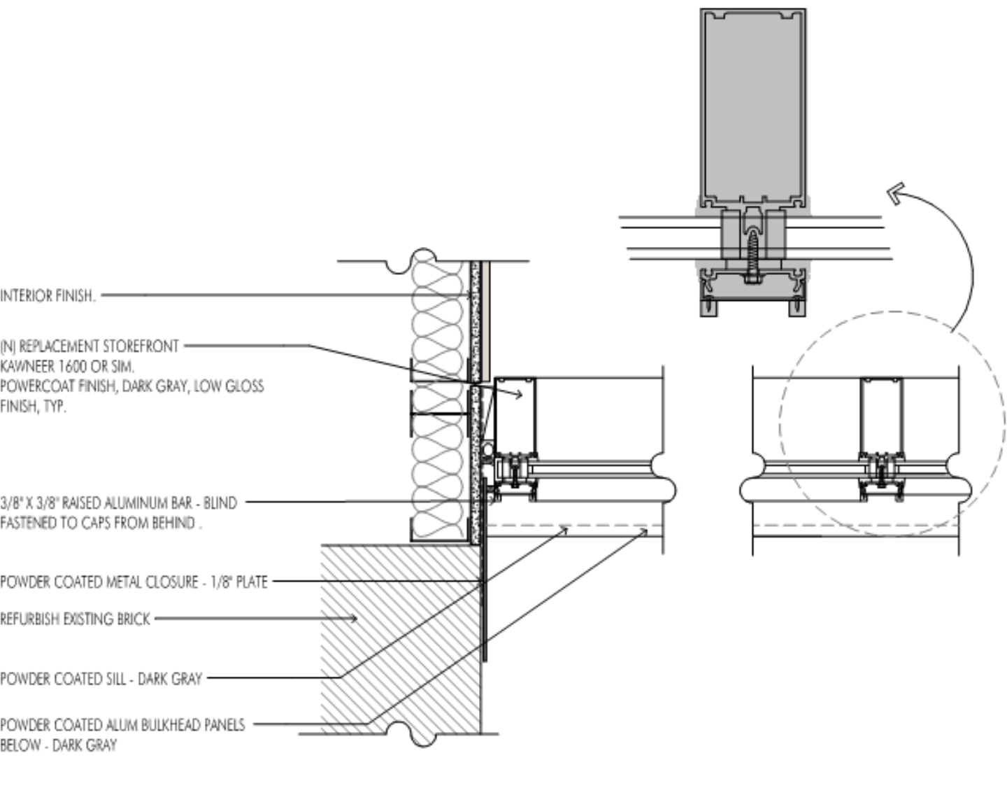
3 17-29 BUILDING JAMB & INTERMEDIATE STOREFRONT DETAIL 3' - 1 1/2"
