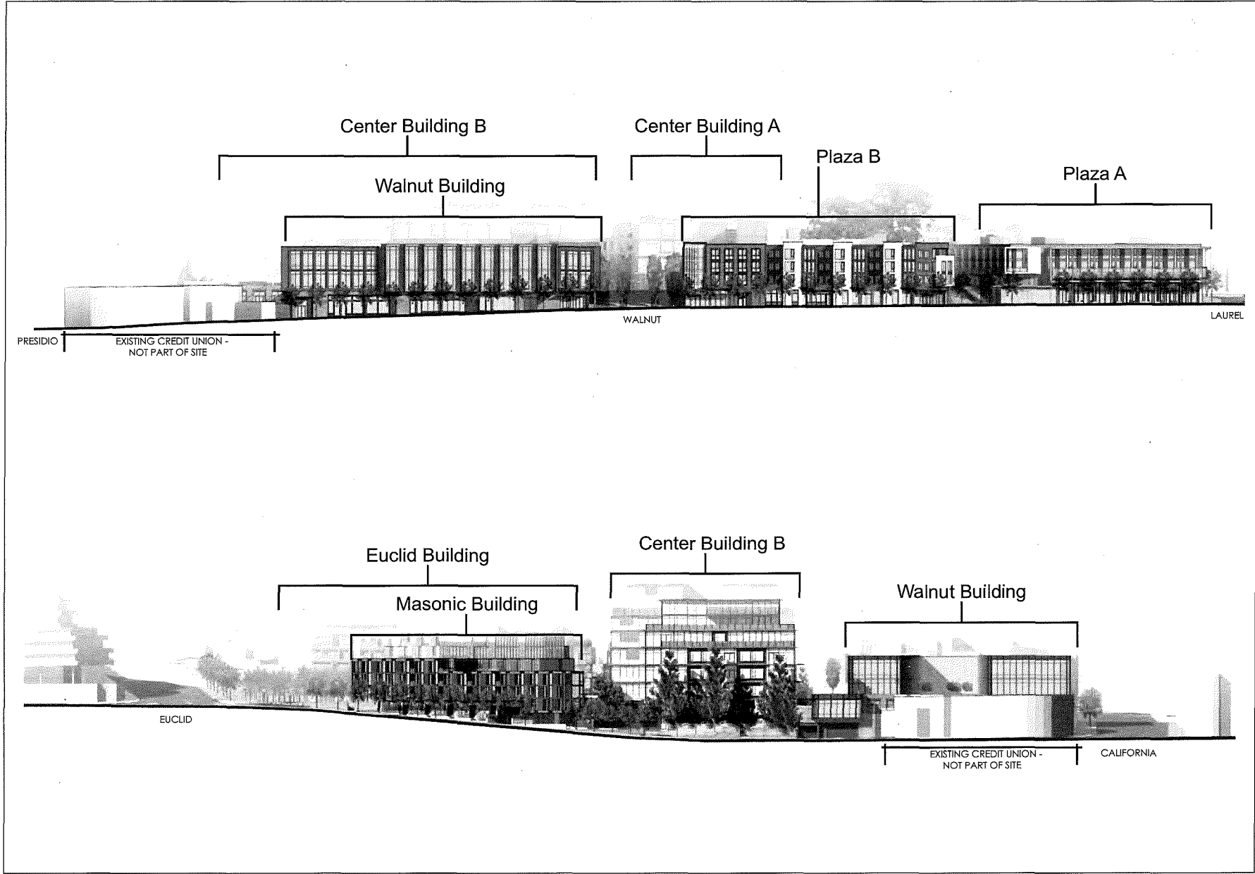
FIGURE 5: PROPOSED CALIFORNIA STREET AND PRESIDIO/MASONIC AVENUE ELEVATIONS
