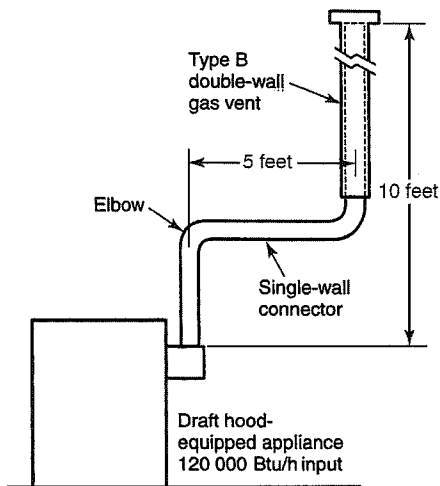
»» FIGURE G 101.3 SINGLE DRAFT HOOD-EQUIPPED APPLIANCE – EXAMPLE 1
