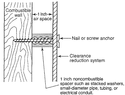
FIGURE 509.7.3(2) WALL PROTECTION REDUCTION SYSTEM [NFPA 54: FIGURE 10.3.2.3(b)]
