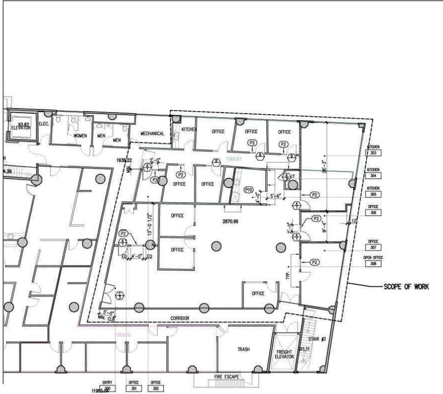
CONSTRUCTION PLAN
