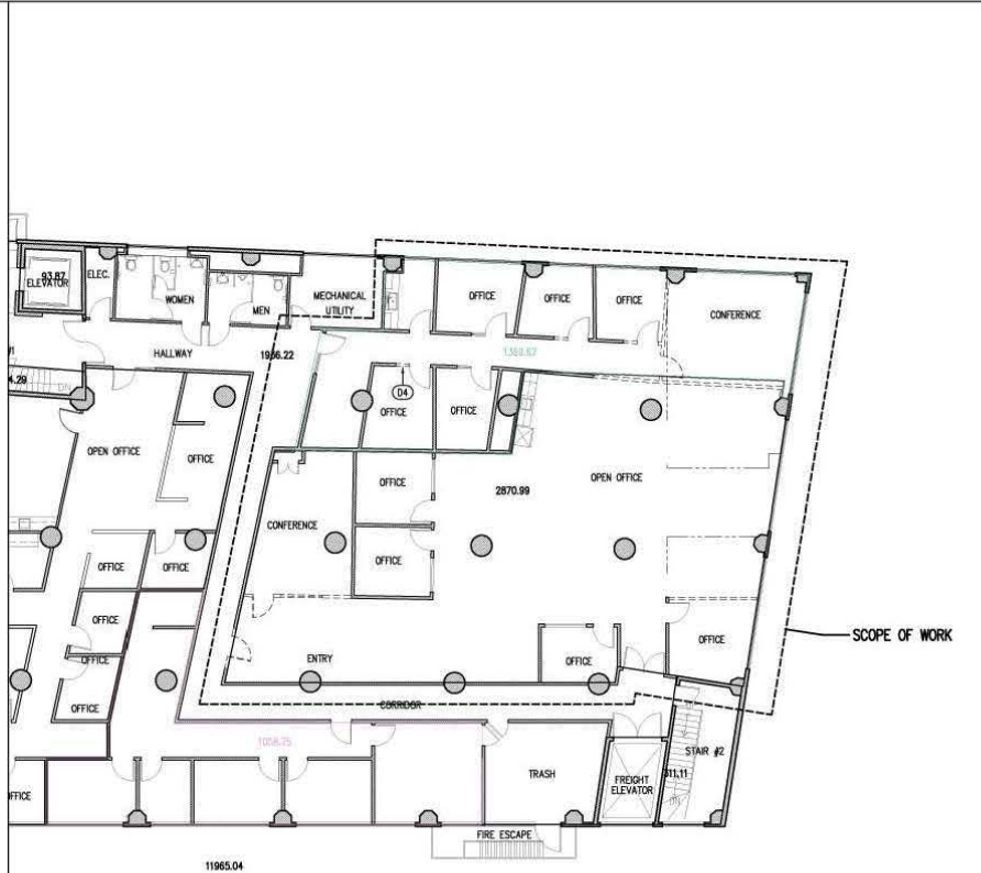
EXISTING/DEMOLITION PLAN
