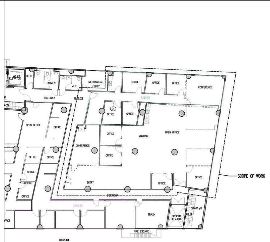
EXISTING/DEMOLITION PLAN
