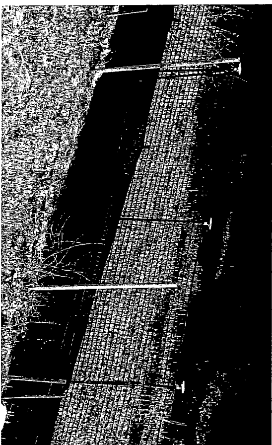
Silt fence is properly installed along the slope to intercept sheet flow.
