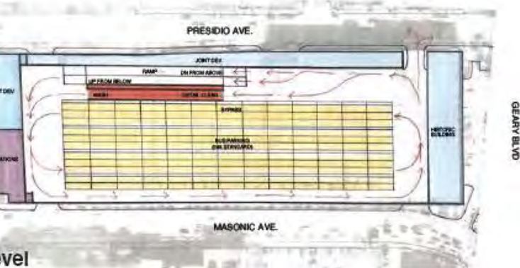
1st Level
