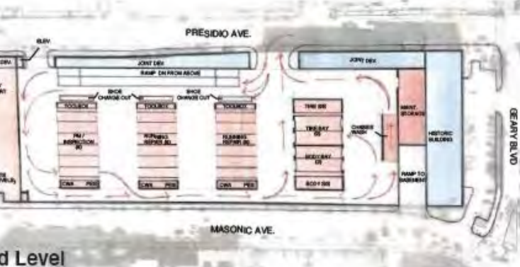
2nd Level
