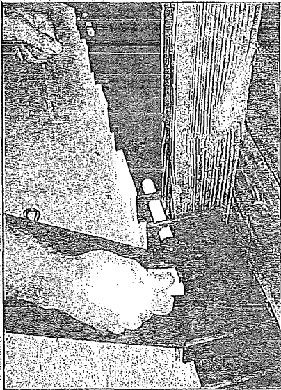
Easy pull pins make rafter replacement easy.
