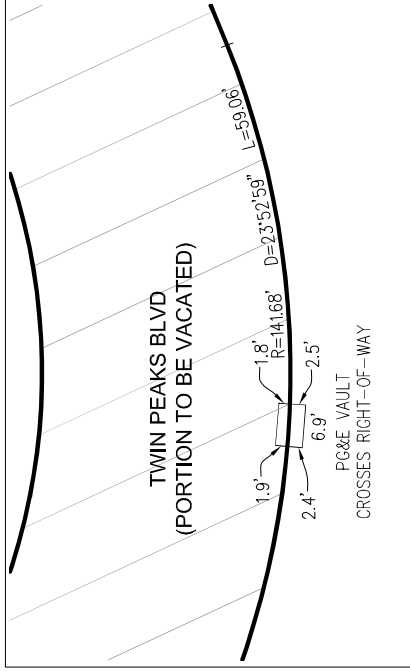
DETAIL D
