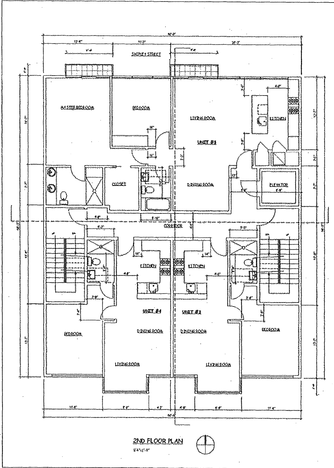
Figure 4. Proposed second floor plan (Source: William Pashelinsky Architect)
