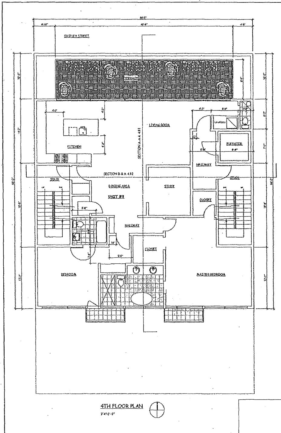
Figure 6. Proposed fourth floor plan (Source: William Pashelinsky Architect)
