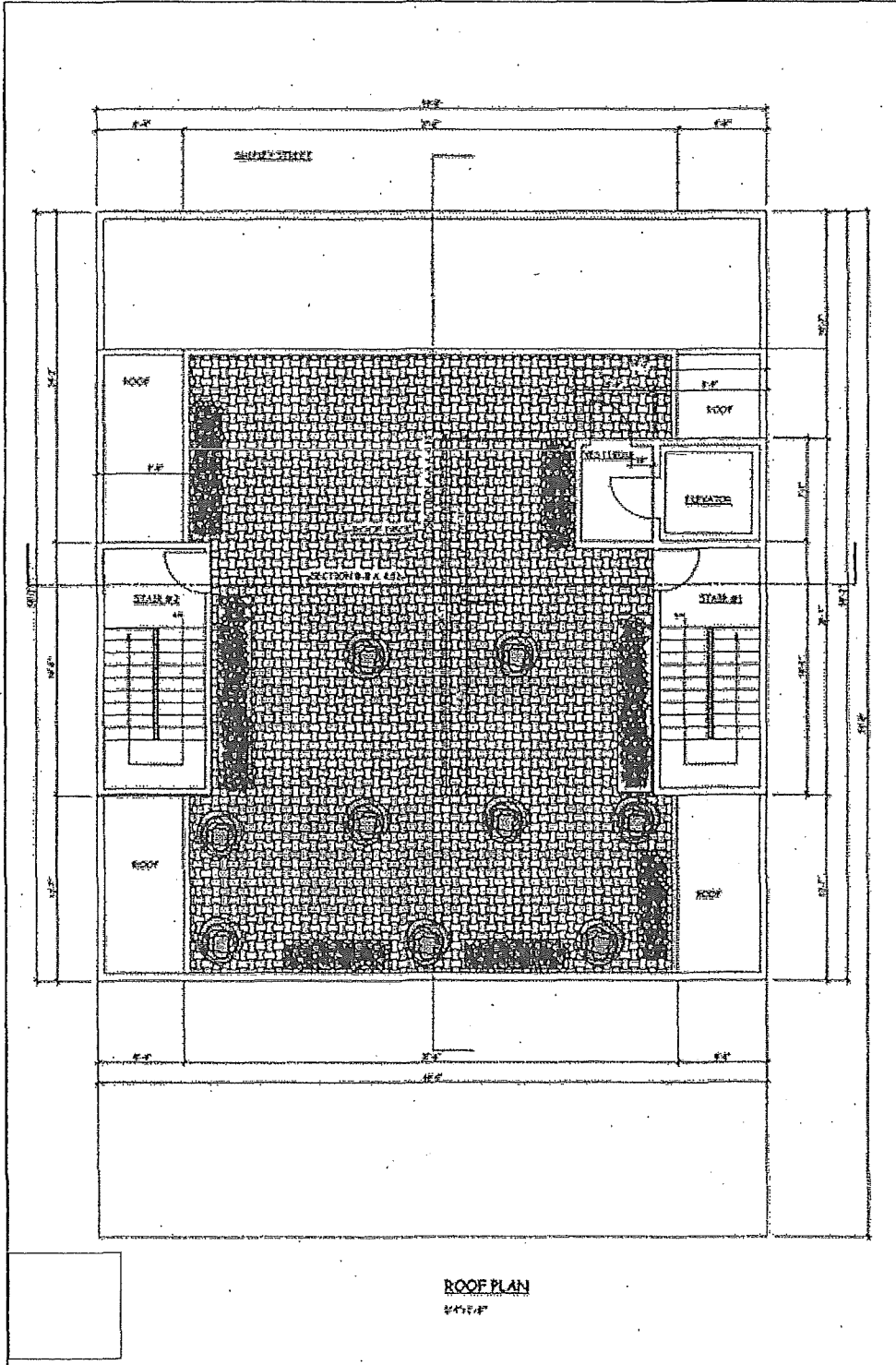
Figure 7. Proposed roof plan (Source: William Pashelinsky Architect)
