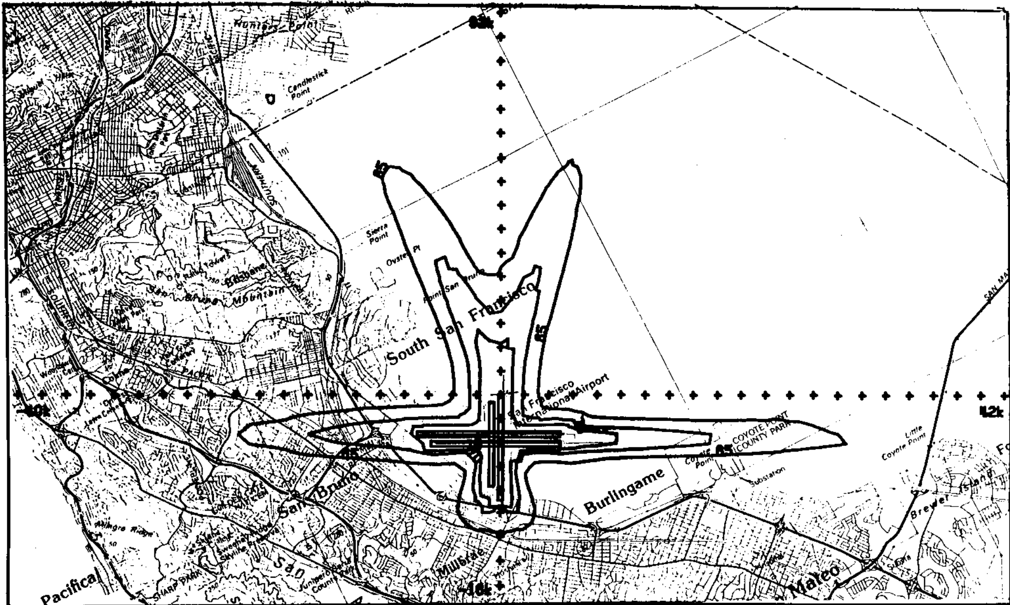
FRA INTEGRATED NOISE MODEL VERSION 8 YEAR 2006 WITH CASP RECOMMENDED SCENARIO SAN FRANCISCO INTERNATIONAL AIRPORT METRIC=CNEL
