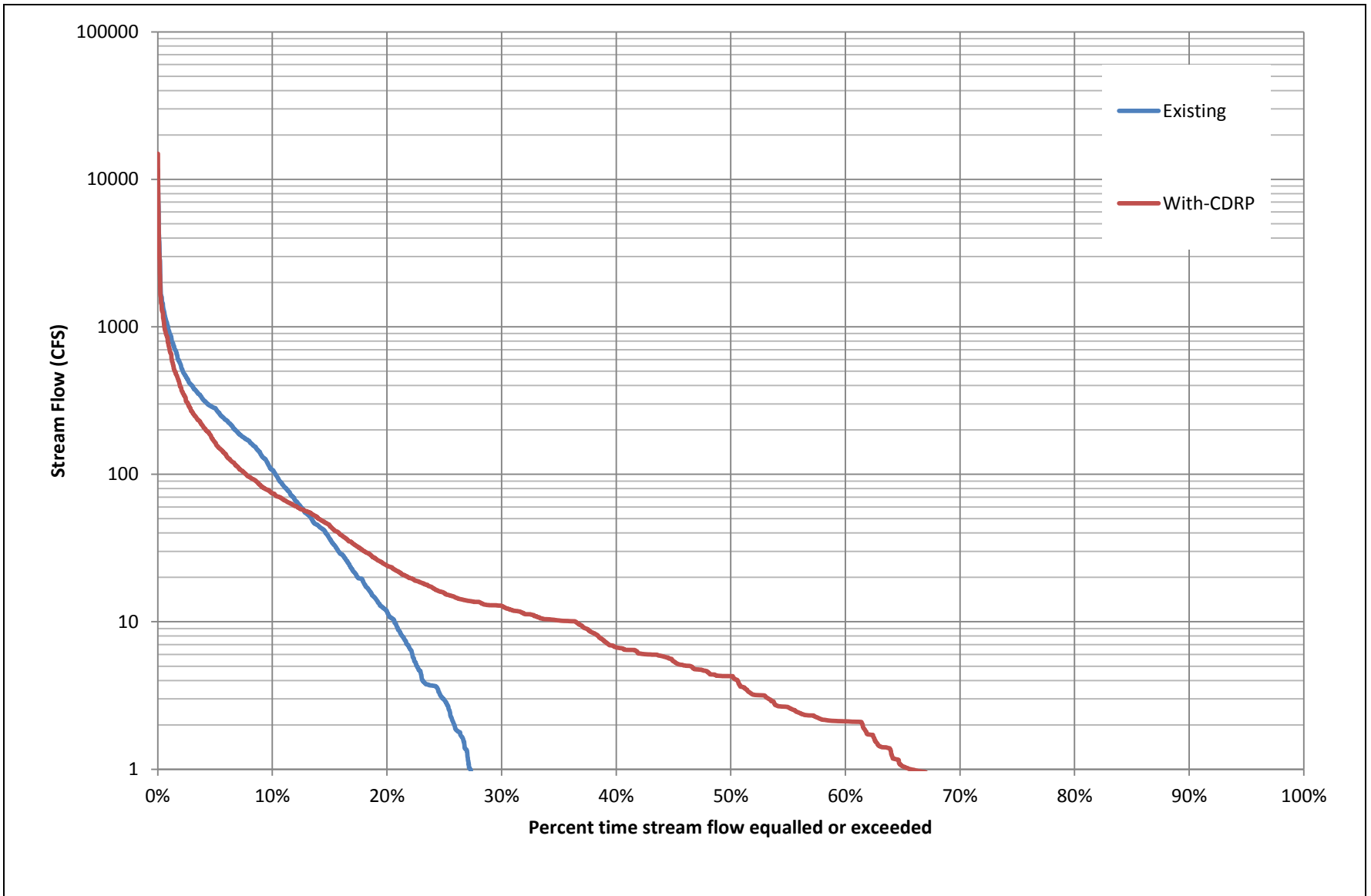
Figure 5.16-5 Flow Duration Curves for Node 7 (Alameda Creek above Arroyo de la Laguna) for Existing and with-CDRP Conditions
