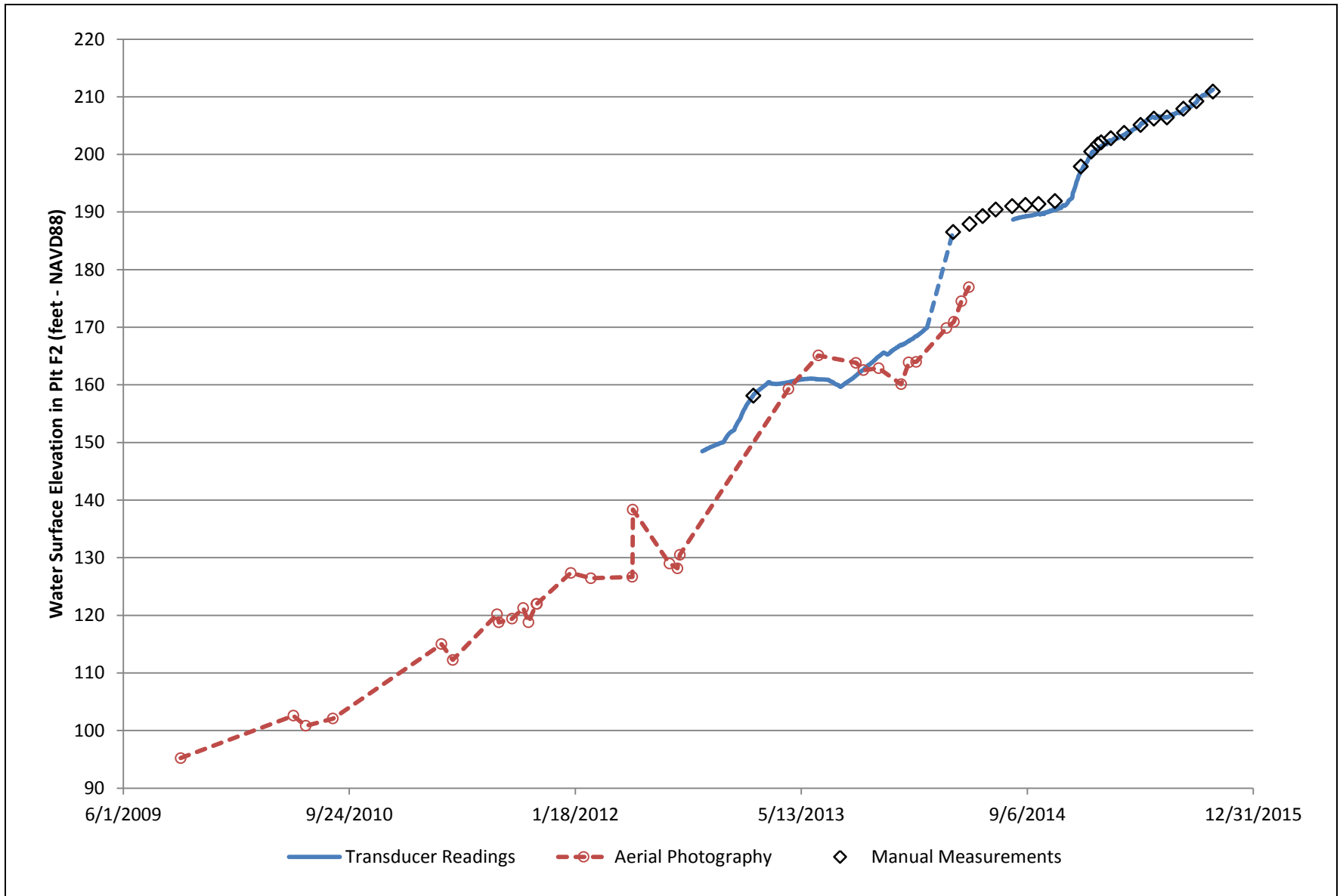
SOURCE: SFPUC, 2015. Pond F2 depth estimation from photo-images during different times. Excel spreadsheet file provided by Amod Dhakal on April 1, 2015; Luhdorff & Scalmanini, 2015; USGS 2015 Data last downloaded 06/2016 SFPUC Alameda Creek Recapture Project Figure 5.16-7 Historical Water Surface Elevations in Pit F2
