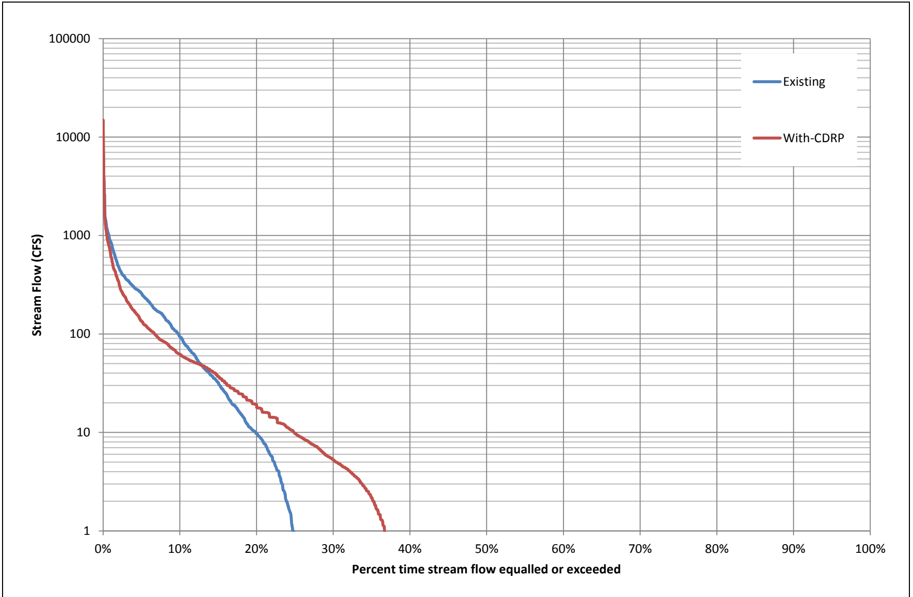
Figure 5.16-4 Flow Duration Curves for Node 5 (Alameda Creek above San Antonio Creek) for Existing and with-CDRP Conditions
