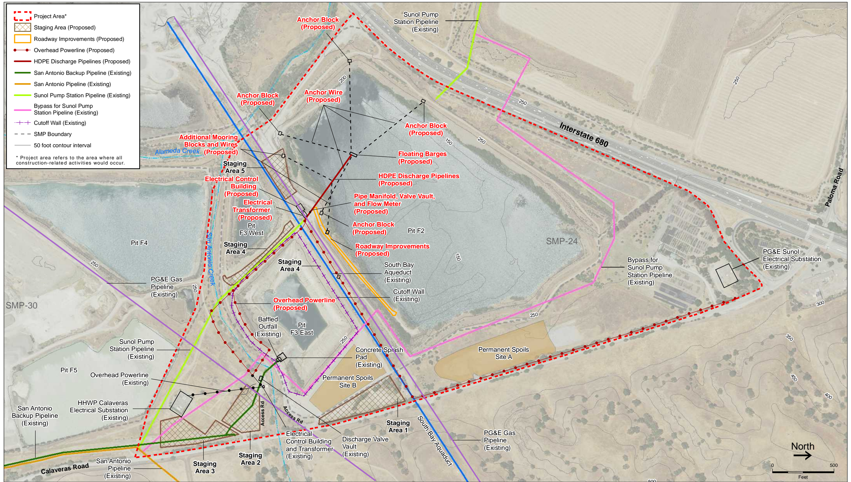
SFPUC Alameda Creek Recapture Project Figure 1-2 Preliminary Site Plan
