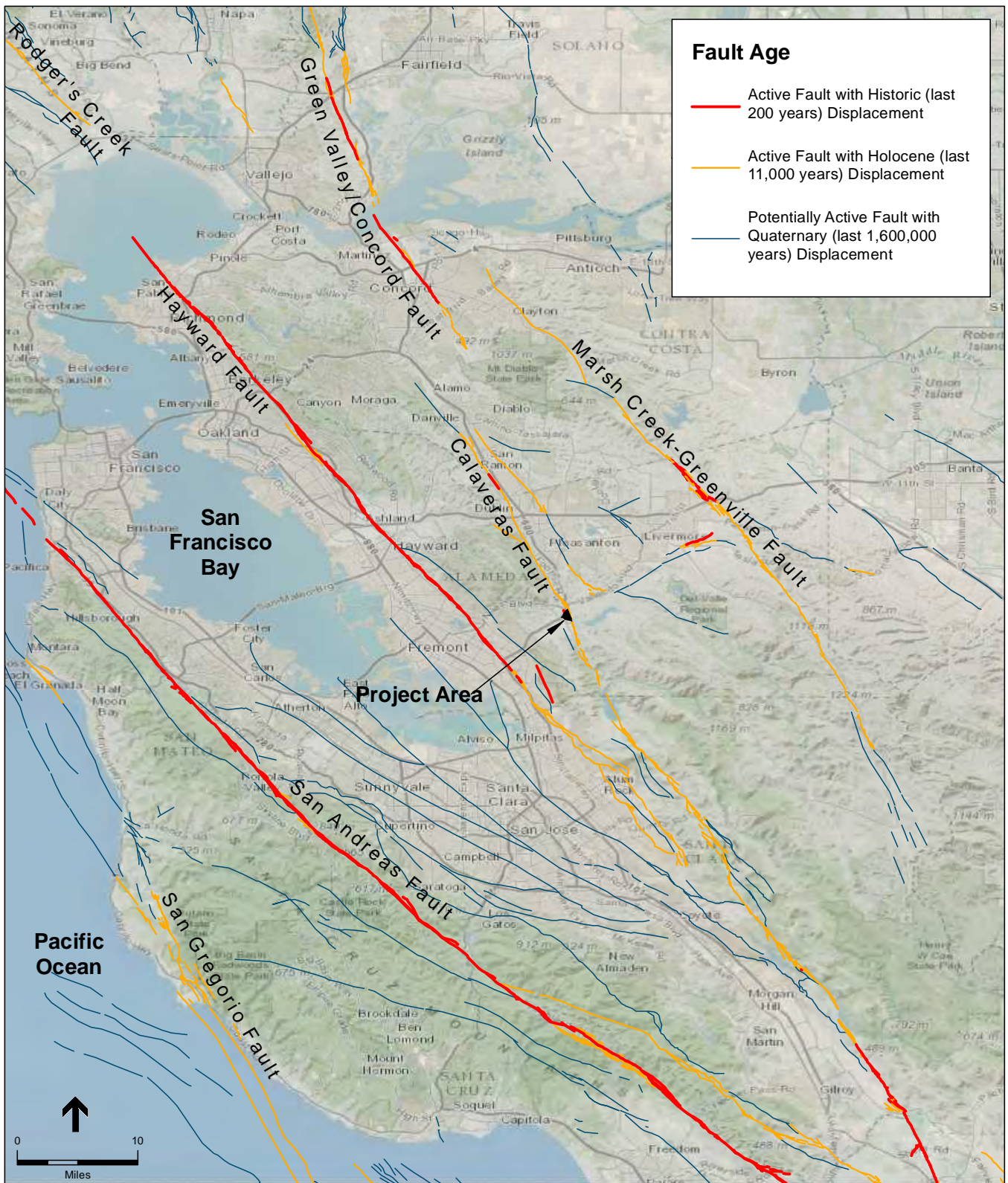
SFPUC Alameda Creek Recapture Project Figure 5.15-3 Major Regional Faults
