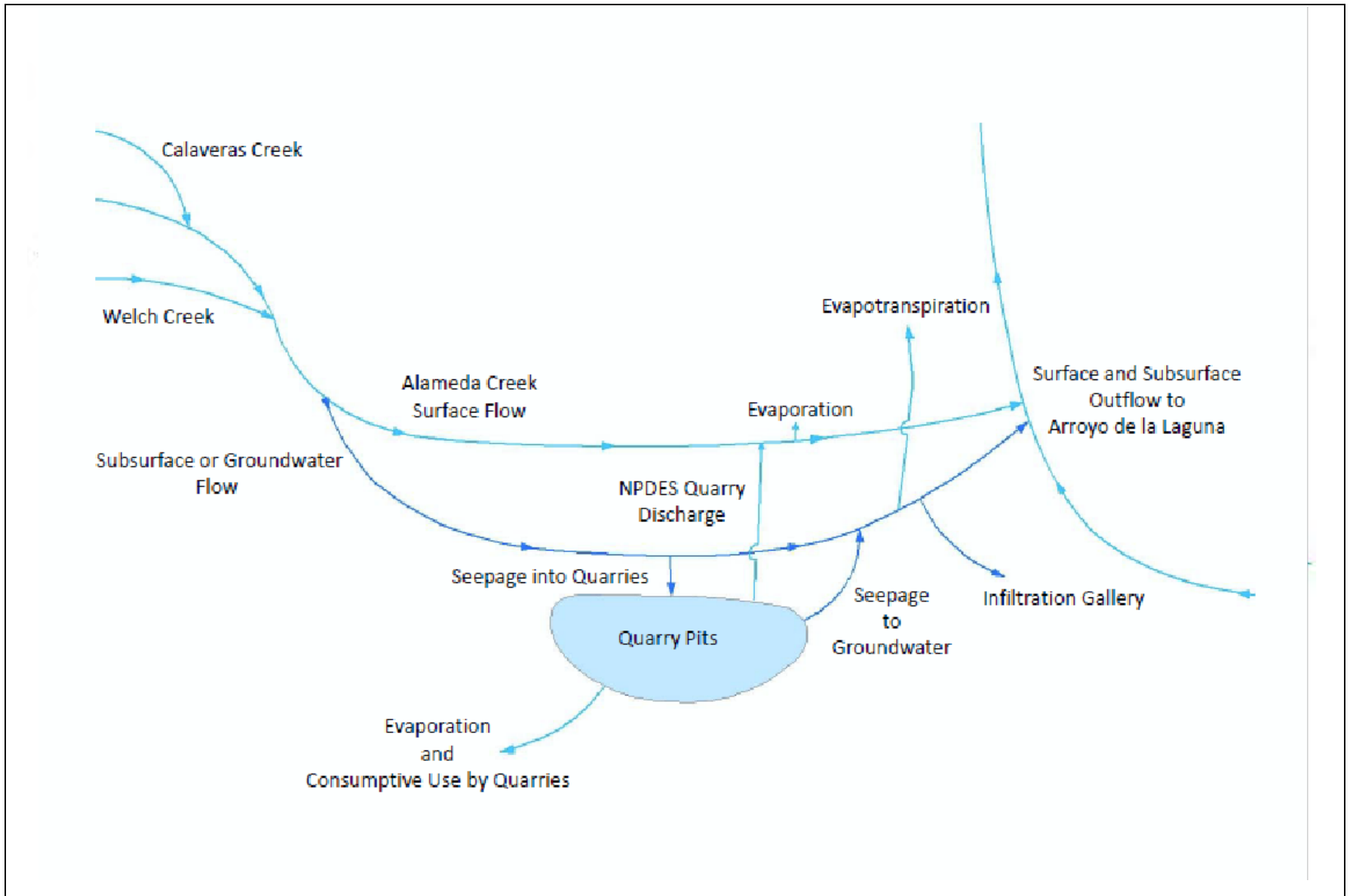
Figure 5.16-19 Groundwater-Surface Water Pathways in the Project Area
