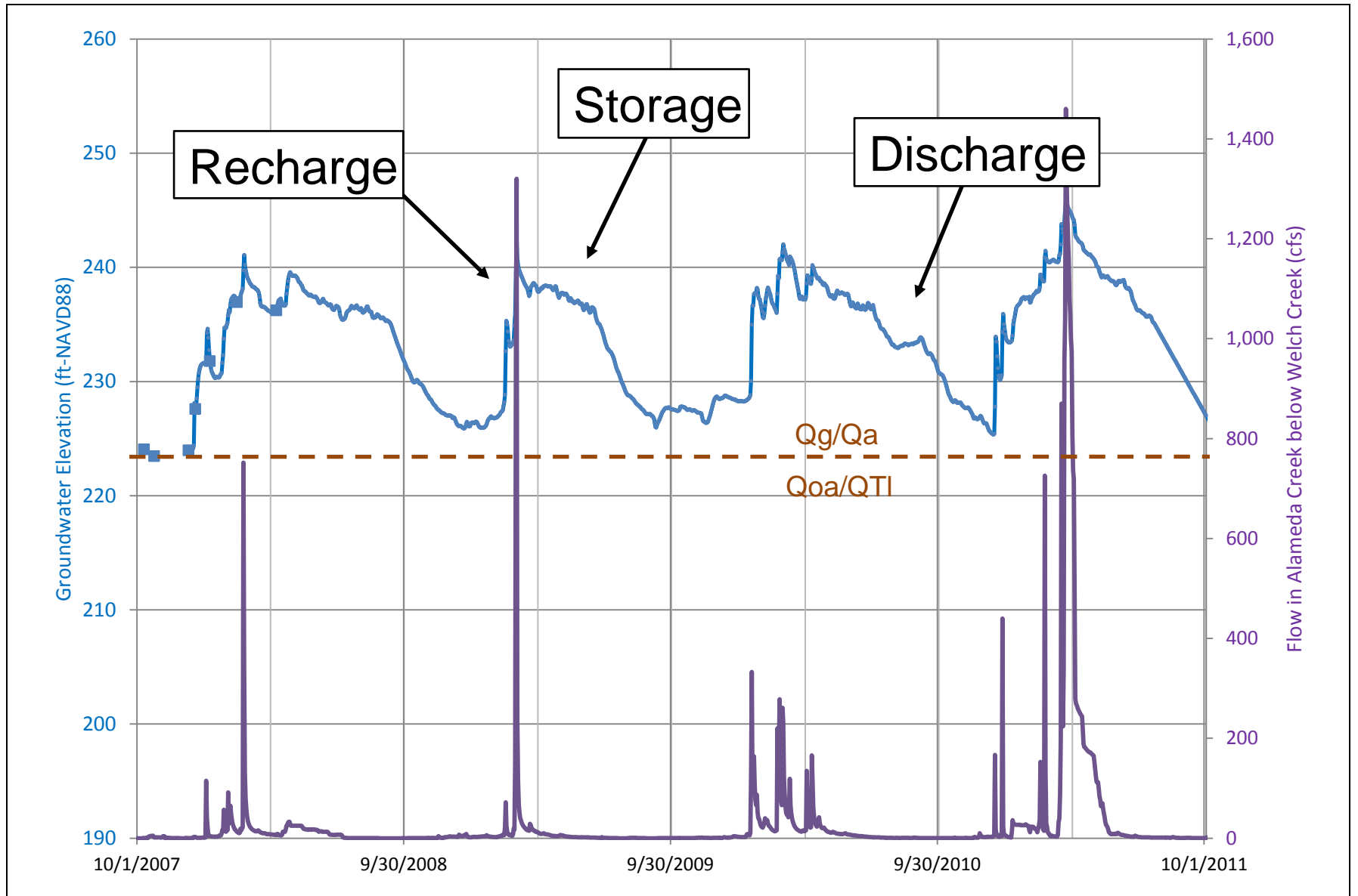
Figure 5.16-16 Hydrograph showing Recharge, Storage, and Discharge Processes
